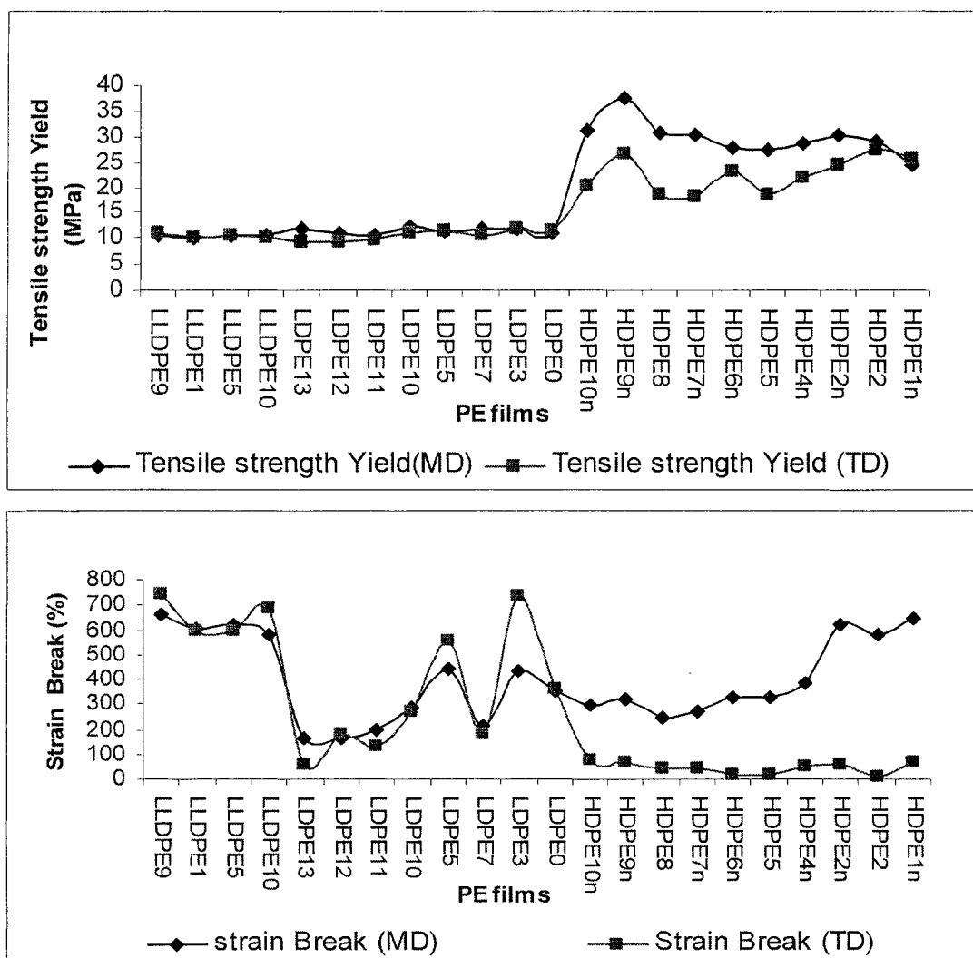
Figure 4.11. Measured mechanical properties.
