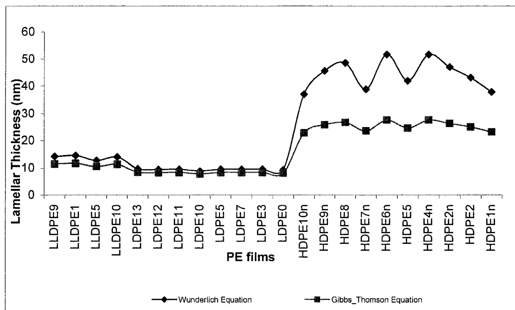
Figure 4.10. Measured lamellar thickness from two different equations.
