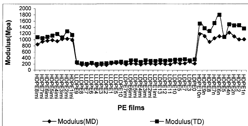
FIG 6.4. Measured tensile modulus
