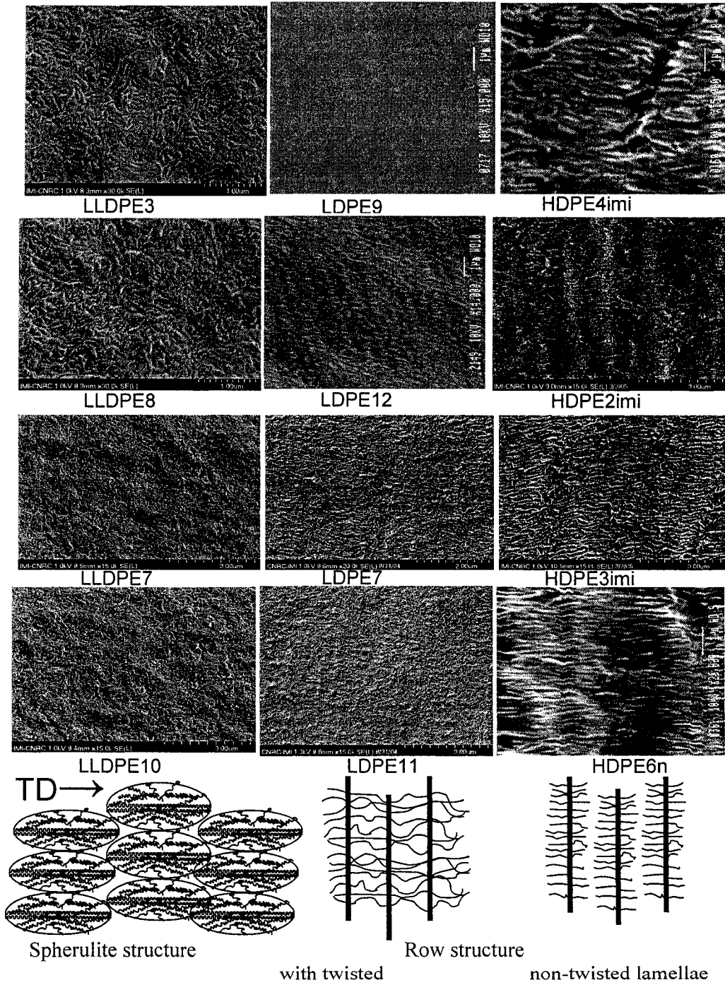
Figure 5.1. Crystalline morphology of surface of different PE blown films.
