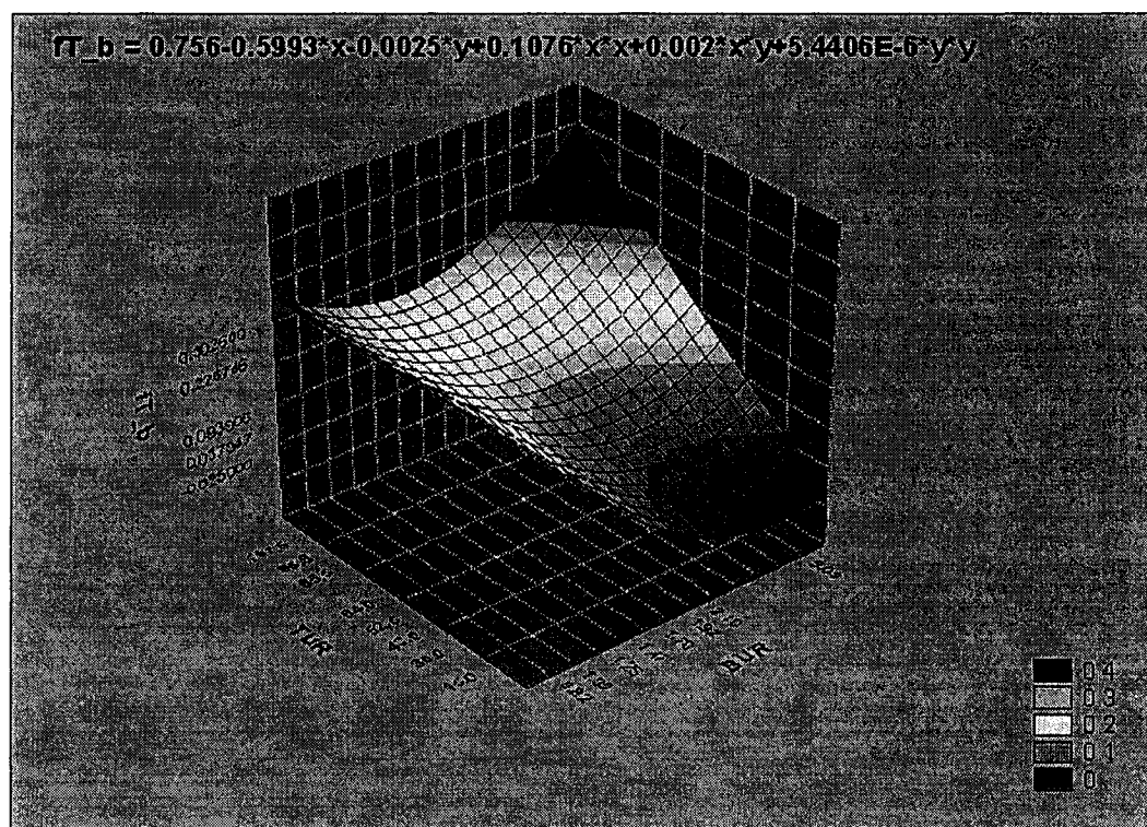
Figure 5.8. Response surface for ft_b ; TUR and BUR as independent variables.
