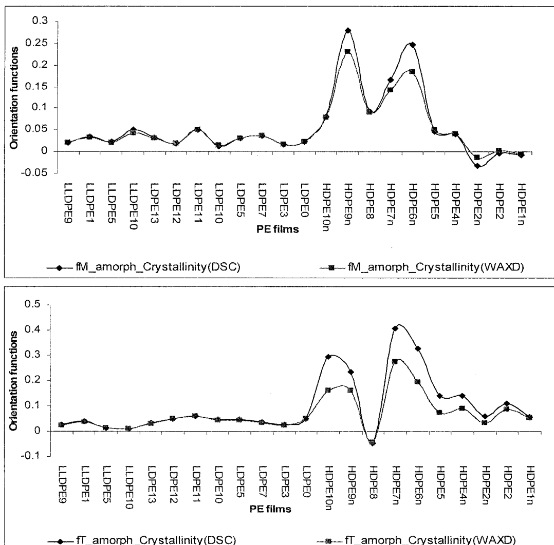
Figure 4.9. Amorphous orientation functions obtained using crystallinity from DSC and WAXD techniques.
