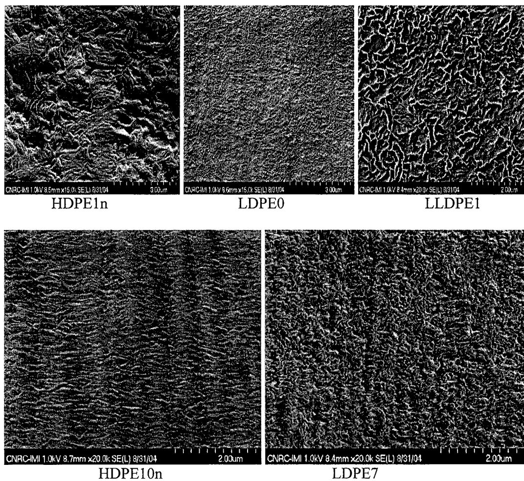
Figure 4.2. SEM images of blown PE films (Machine Direction↑, Transverse Direction→).
