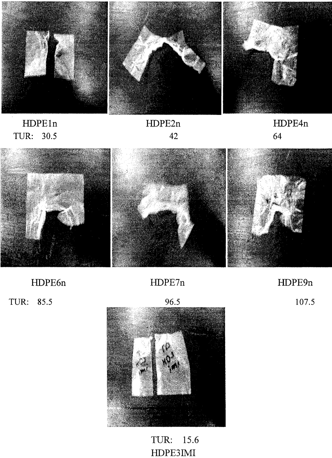
Figure 5.7. Photographs of the TD tear strength failure samples ((TD↑, MD→).
