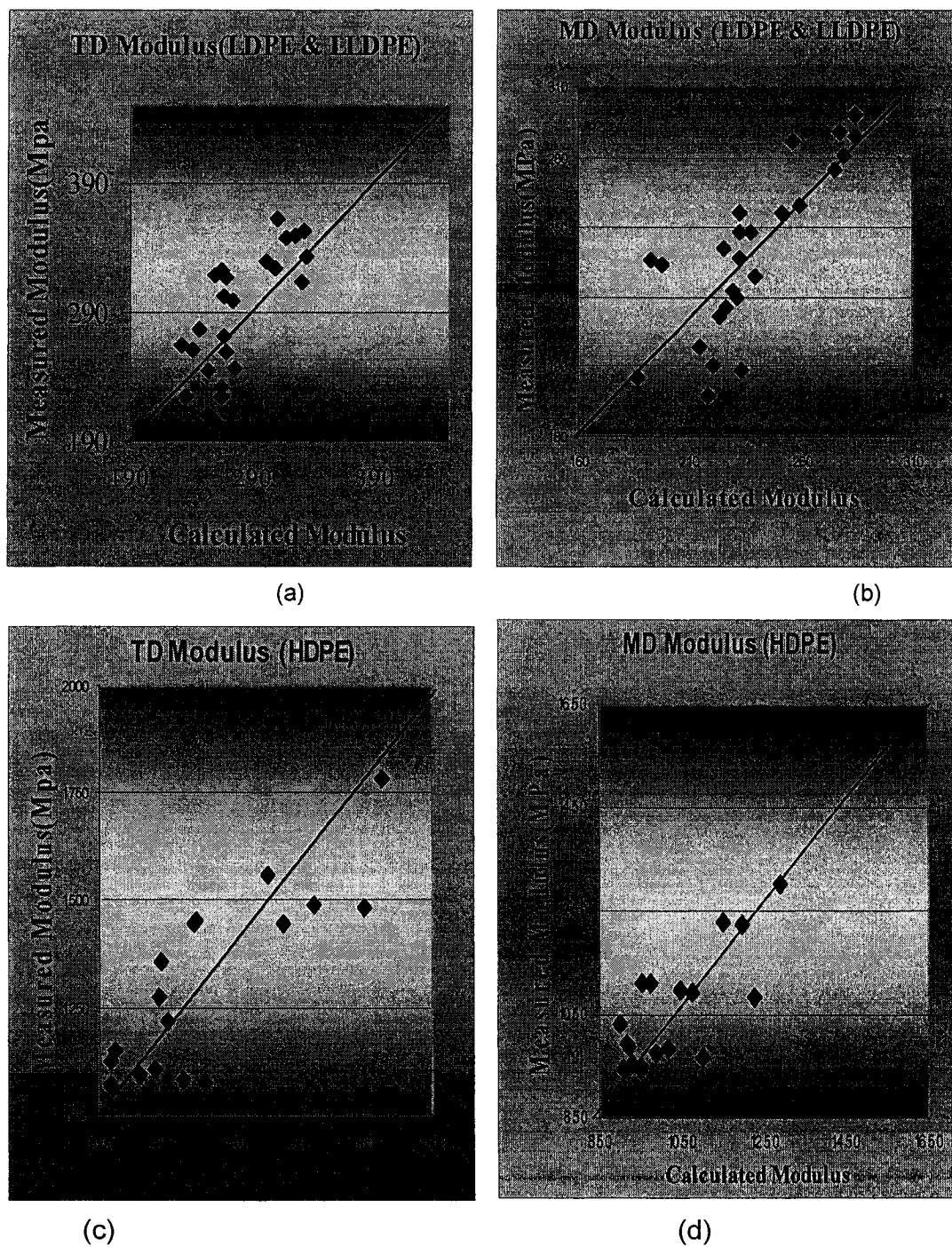
FIG 6.11. Predicted and measured modulus of different PE films
