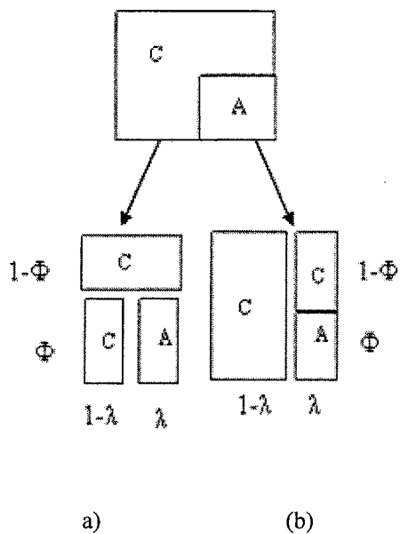
FIG 6.9. Takayanagi models for polymer blends.
