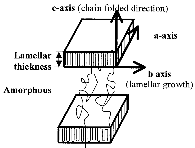
FIG 6.7. The folded chain mode in PE
