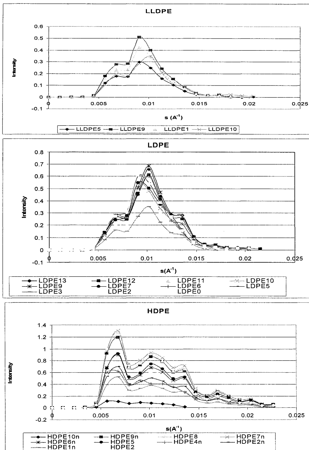
Figure 4.6. SAXS intensity distribution curves for LLDPE, LDPE, and HDPE films.
