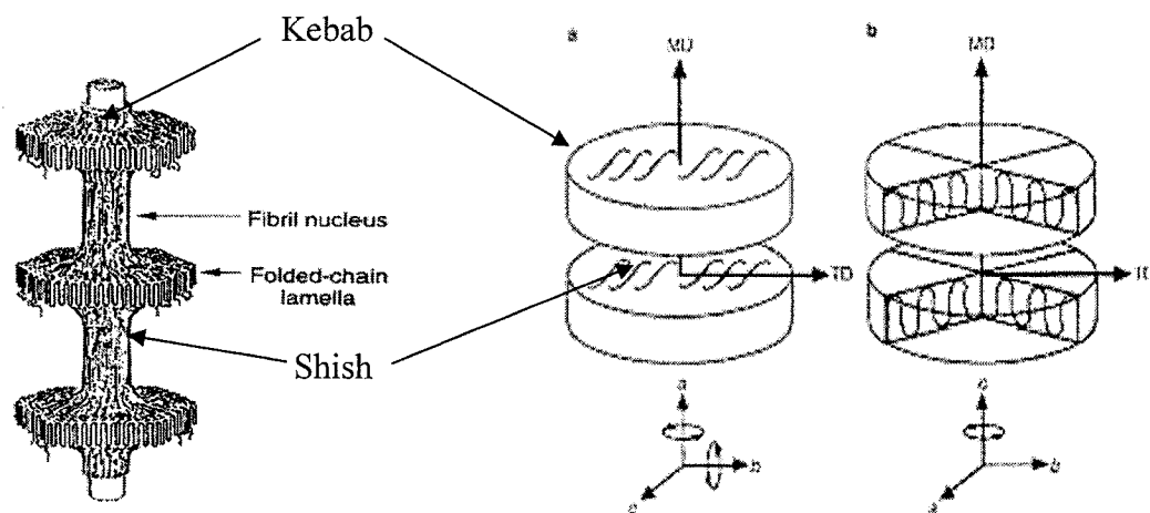
Figure 2.1. Shish-kebab morphology
