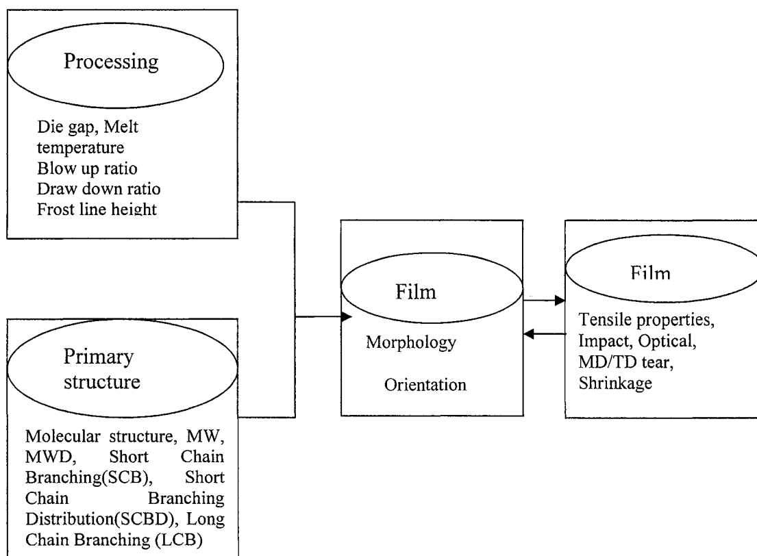
Figure 4.1. Schematic of effects of the structure and processing conditions on the mechanical properties.
