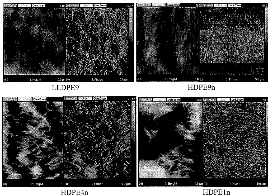
Figure 4.3. AFM images of the surfaces of blown films.
