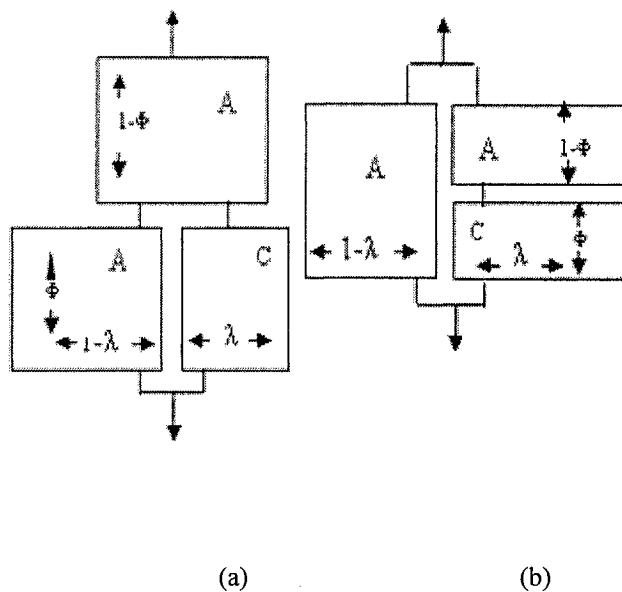
FIG 6.10. The series-parallel(a) and parallel-series (b).
