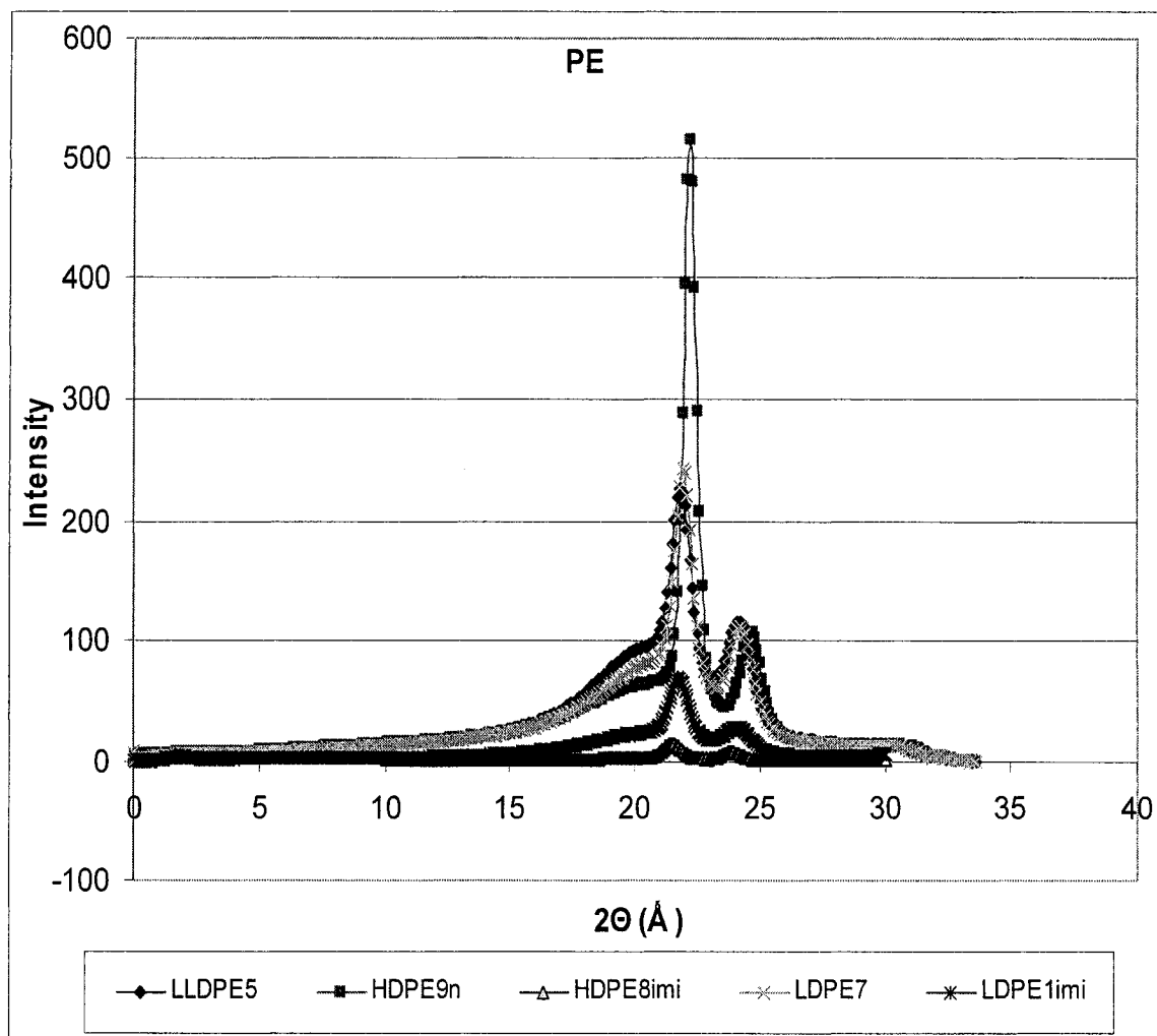
FIG. 6.1. WAXS profiles for PE blown films
