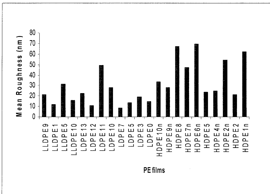
Figure 4.5. The surface roughness of the samples measured by AFM.
