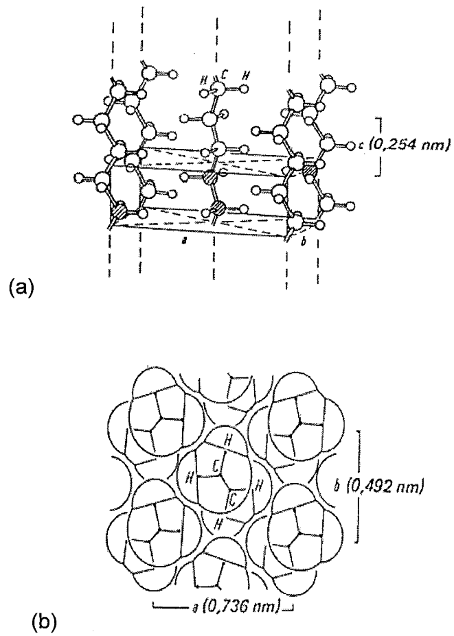
FIG 6.6. Arrangement of the polymer chains in (a) a polyethylene single crystal and (b) View along the C-direction
