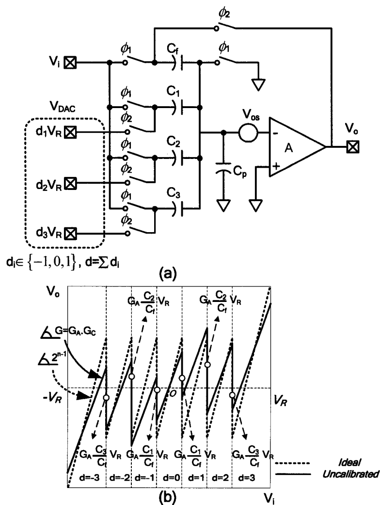
Figure 5.3: MDAC implementation for 2.5 bit/stage pipelined (a), and the residue plot of a realistic stage compared with an ideal one (b)
