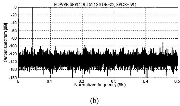
Figure 5.11: Spectrum of the output of a 14-bit pipelined ADC without (a) and with the proposed calibration technique (b).
