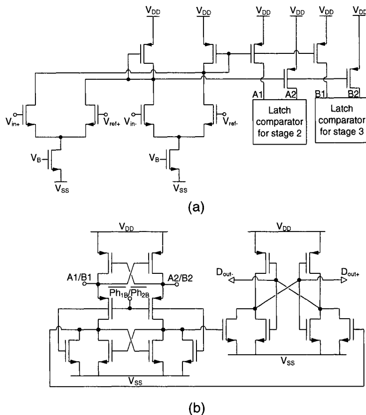
Figure 6.5: Current-mirrored fully differential preamp (a) and latch stage (b).
