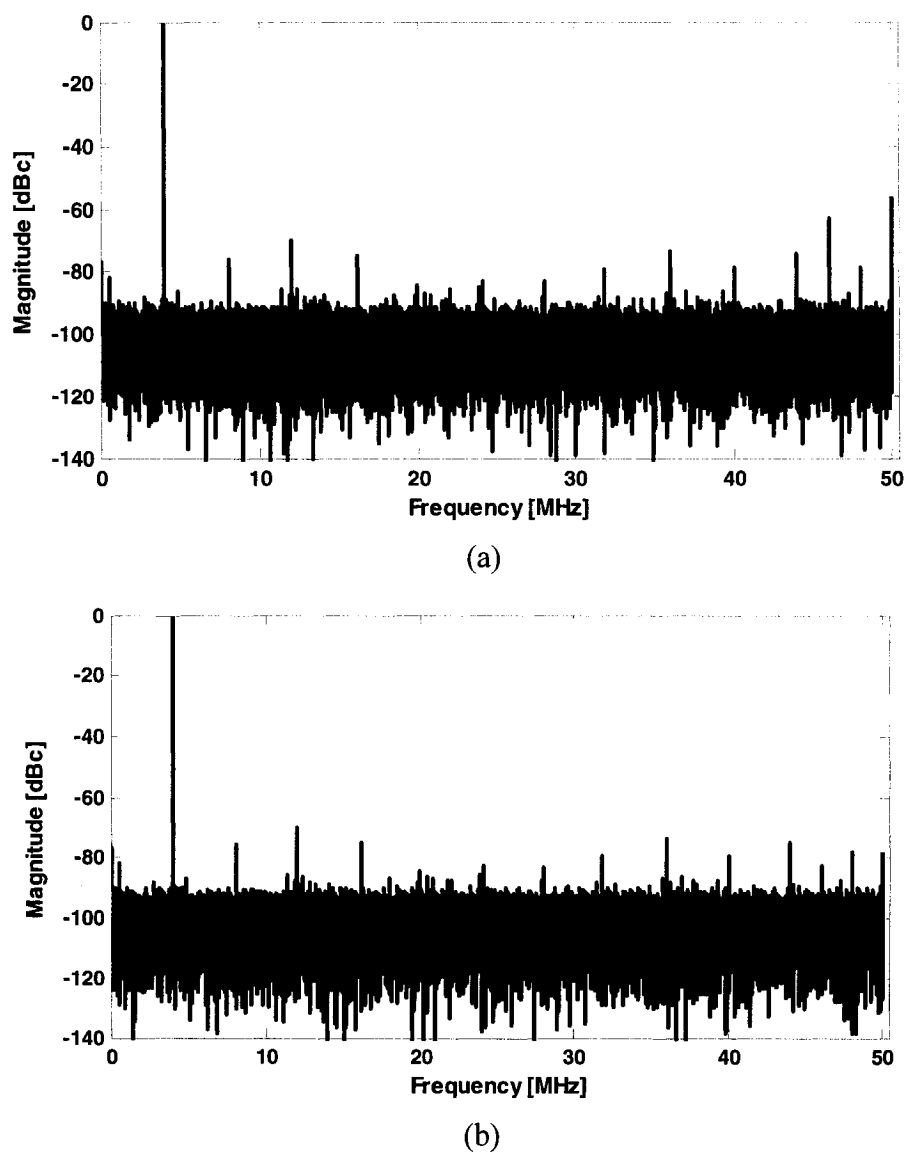
Figure 6.12: ADC output spectrum: (a) without calibration, and (b) with calibration.
