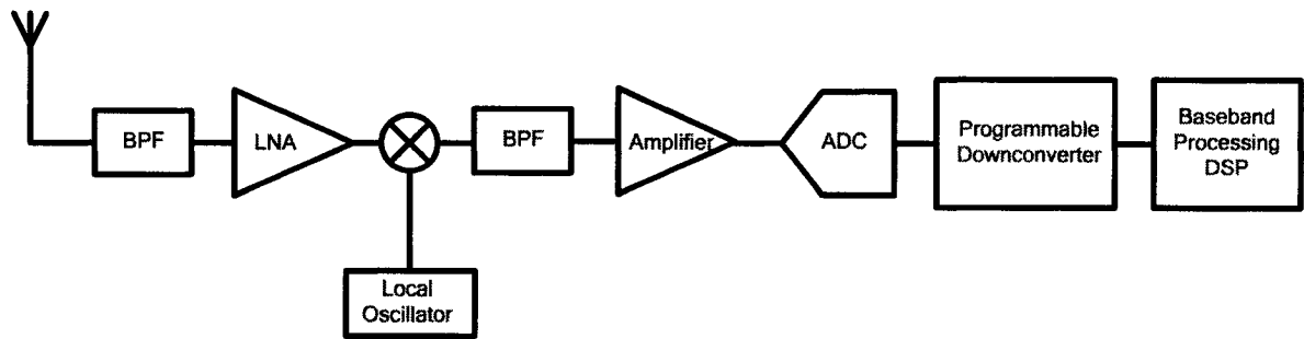
Figure 1.2: The digital radio receiver architecture employing IF-sampling.
