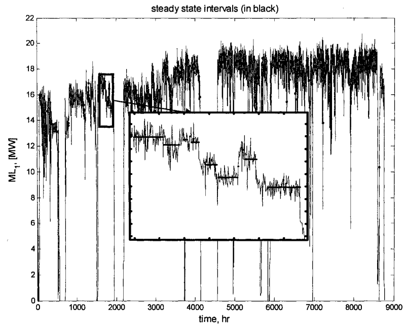
Figure 3.5. Motor load - Primary refiner. Steady state identification.
