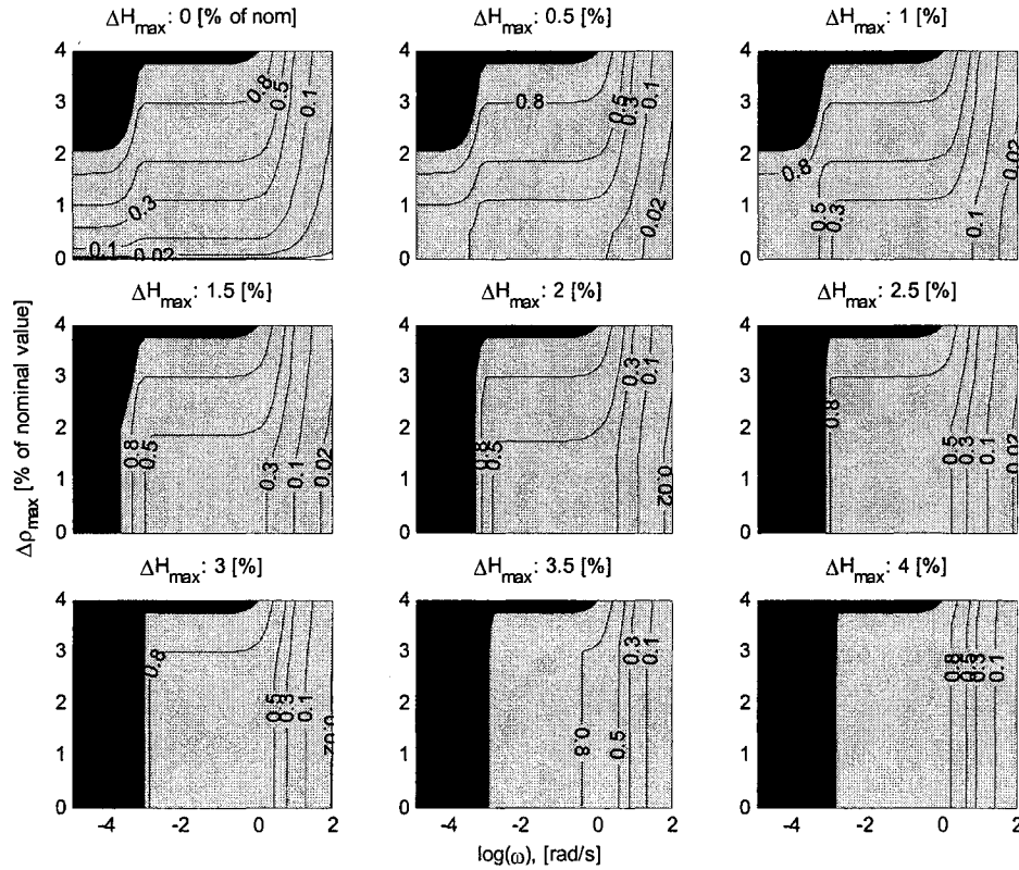
Figure 8.7. Wood variability conditions where control is definitely needed |G_d|_{\max} > 1 (dark areas). Plate age scenario: P602-S602.
