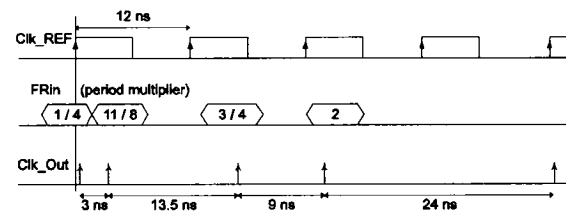
Fig. 1. A timing diagram demonstrating VPCS
