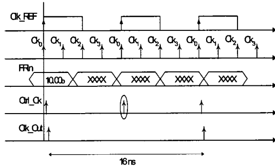
Fig. 5. Period multiplied by an integer: clock division
