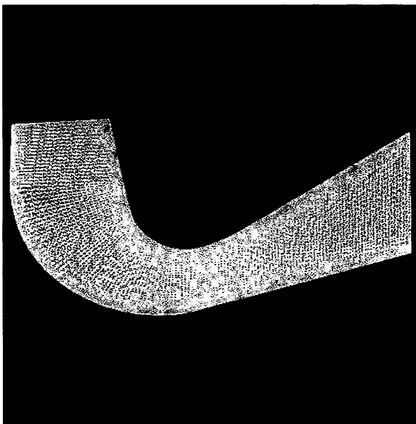
FIGURE 6.24 - Surface originale comportant 30 920 triangles
