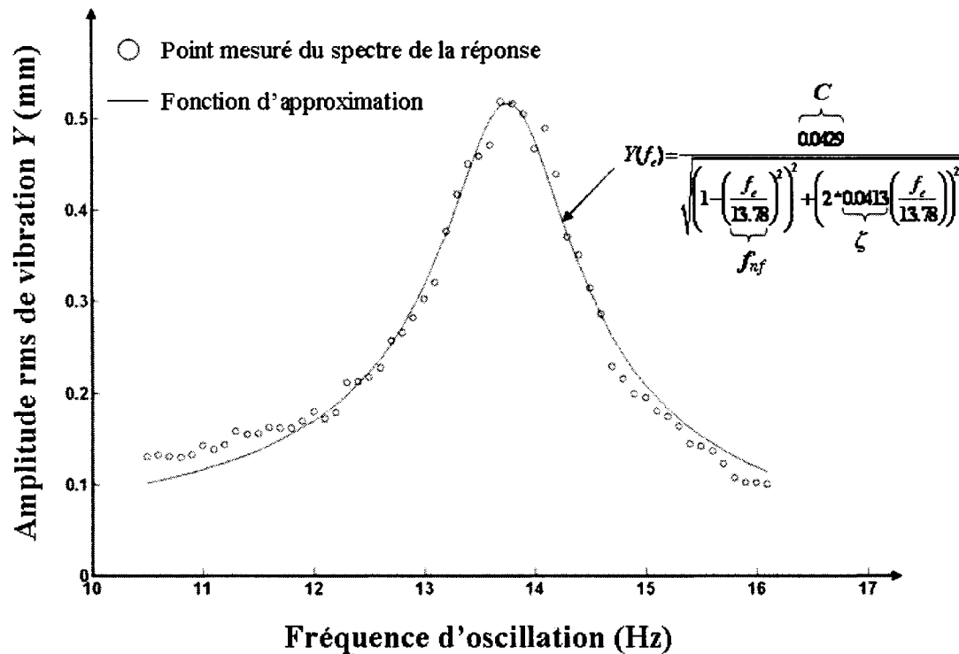
Figure 2.15 Approximation spectrale
