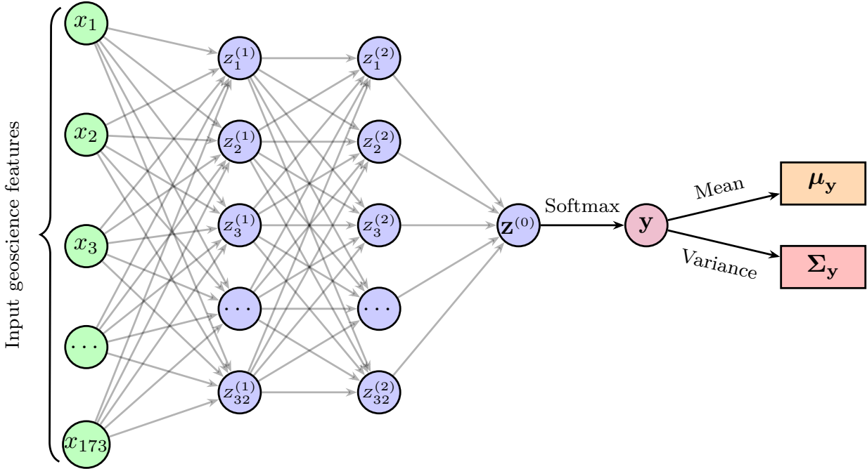
(a) TAGI-MPM architecture illustrating the 173 input geoscience feature vector ( \mathbf{x} = [x_1, x_2, \dots, x_{173}] ) that are processed through two hidden layers ( \mathbf{z}^{(1)} and \mathbf{z}^{(2)} ) of 32 neurons each, followed by an output layer ( \mathbf{Z}^{(0)} ) which contains logits for binary prospectivity classification (barren vs. mineral). The hierarchical softmax activation produces a single probabilistic observation output \mathbf{y} . From this output distribution, we can then derive the prospectivity score \mu_{\mathbf{y}} and its associated uncertainty \Sigma_{\mathbf{y}} .
