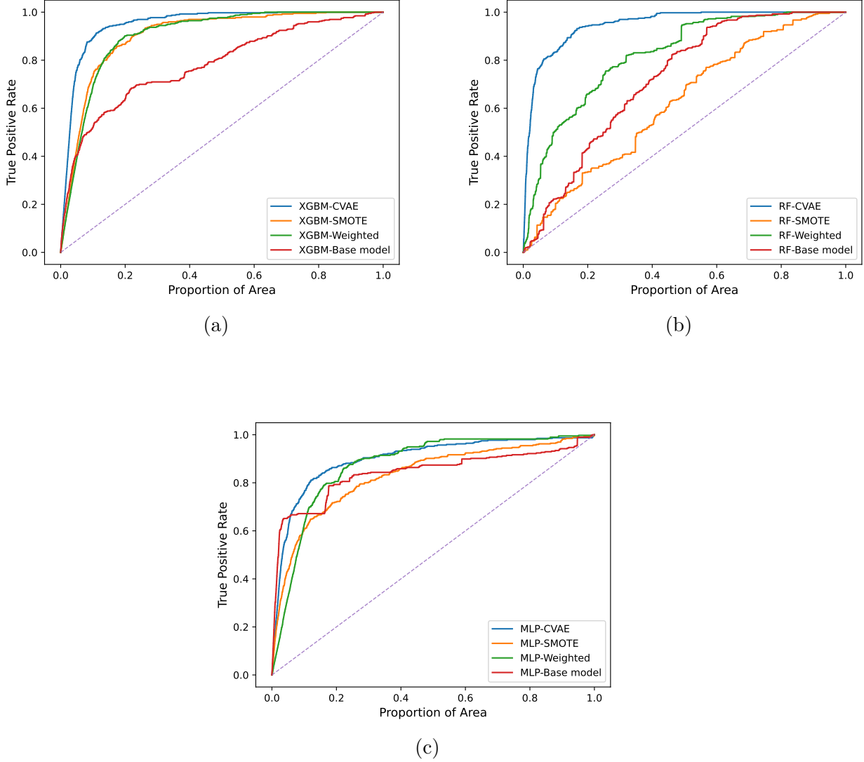
Figure 4.6 Success rate curves for the testing data set with (a) XGBM-MPM, (b) RF-MPM and (c) MLP-MPM models. The dashed lines are the success rate curves characteristic of a random classifier.
