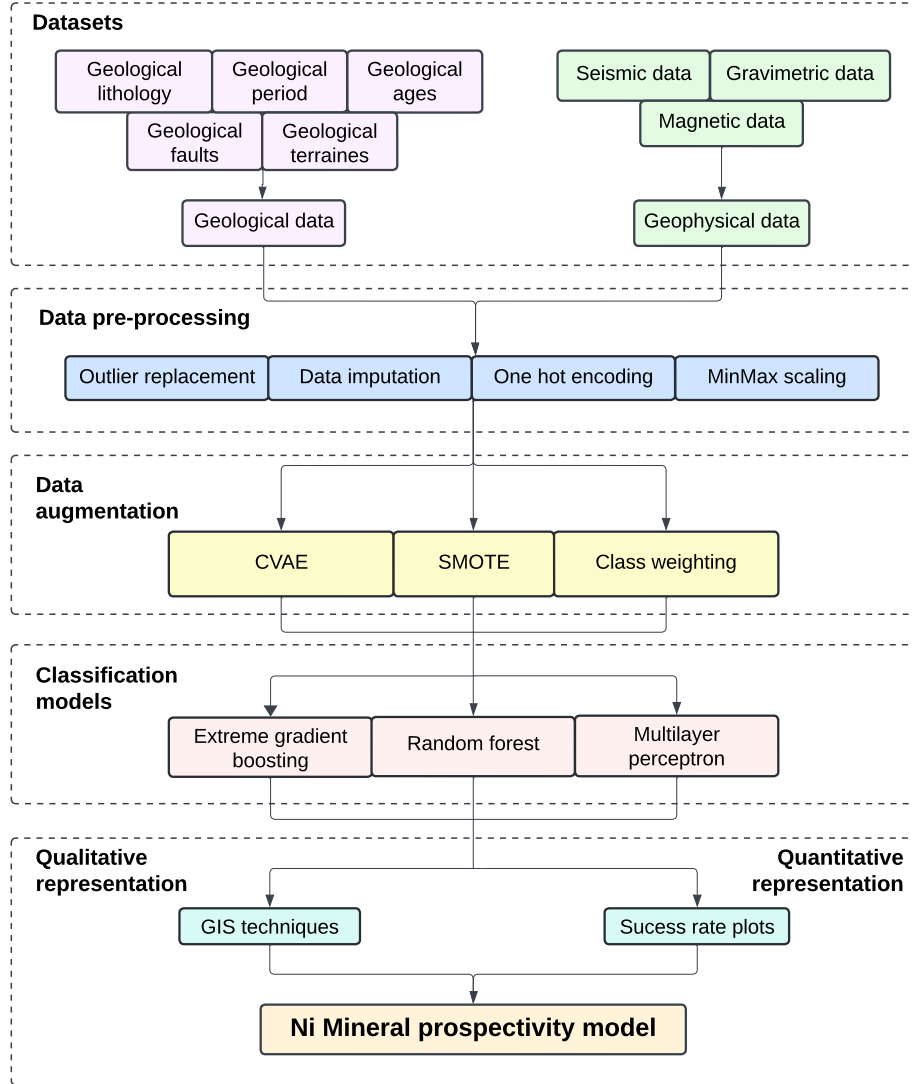
Figure 4.4 Flowchart of the proposed framework of this study.
