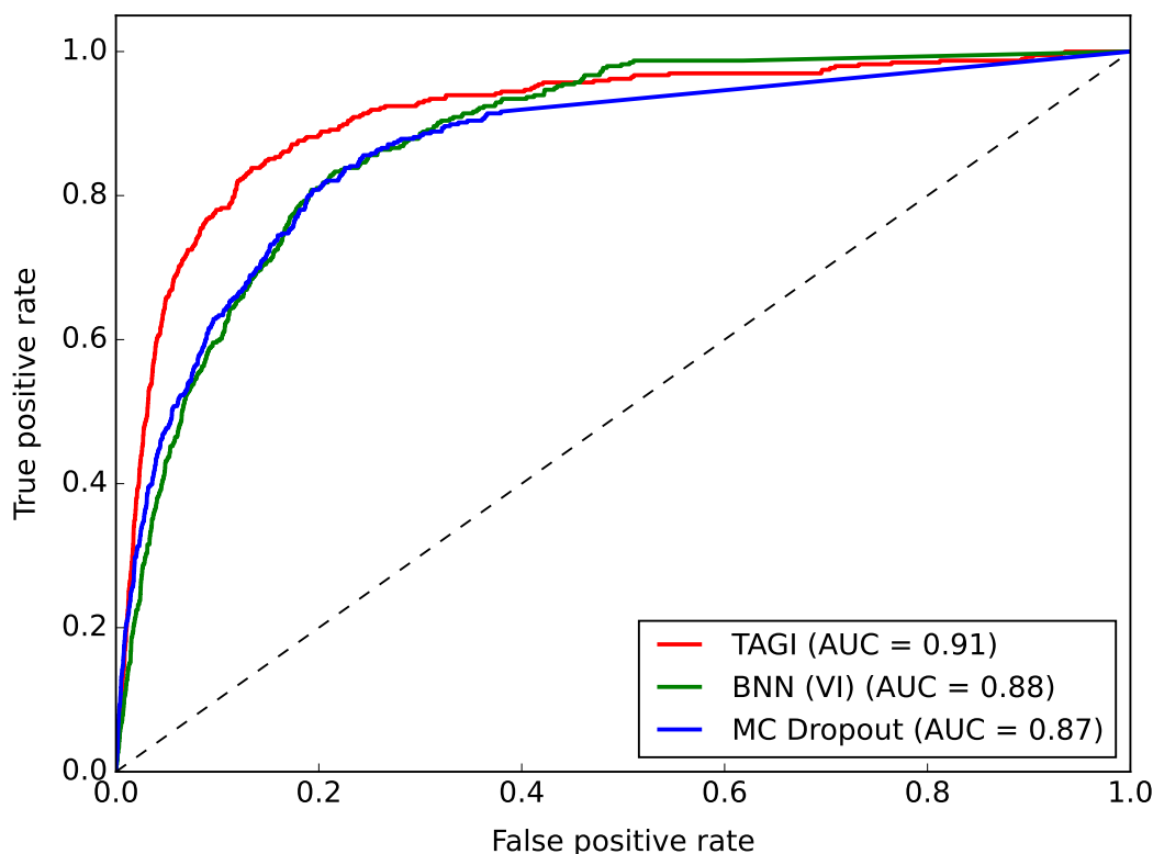
Figure 6.4 Mean ROC curves and AUC values for the TAGI, BNN with VI, and MC dropout models on the unseen test set. The dashed diagonal line represents the performance of a random classifier with an AUC of 0.5.
