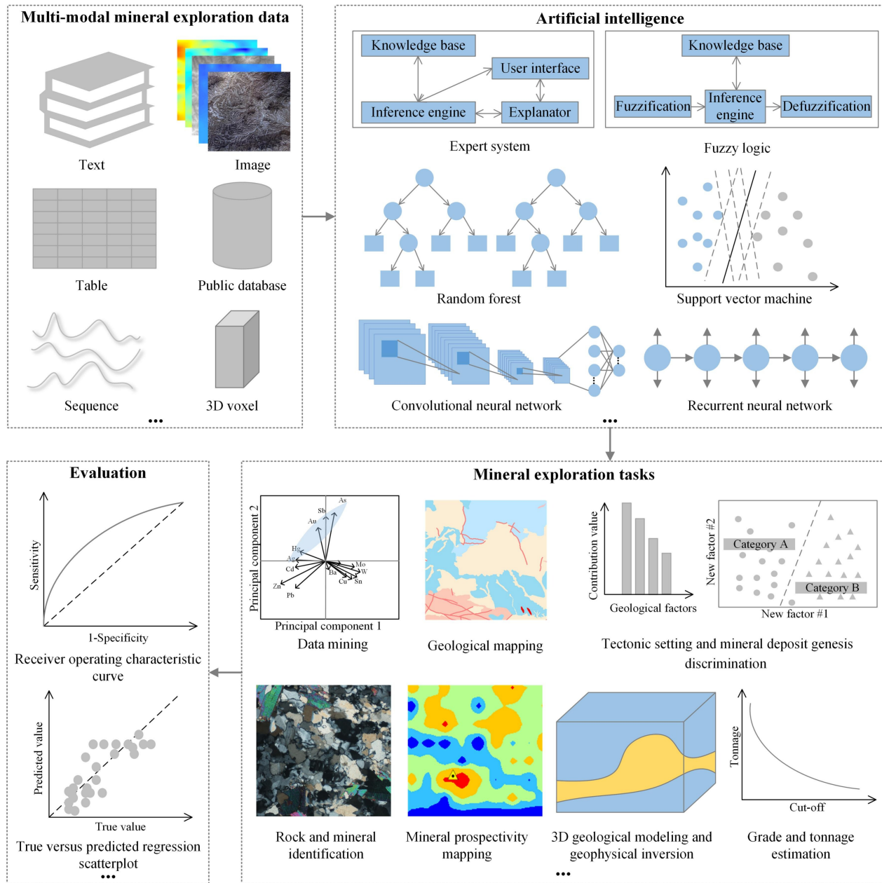
Figure 2.4 Conceptual workflow illustrating the use of AI in mineral exploration. The process usually involves acquiring geoscience datasets, constructing AI models, applying these models to specific exploration tasks such as mapping, classification, or prospectivity analysis, and evaluating their performance (Yang et al., 2024a).
