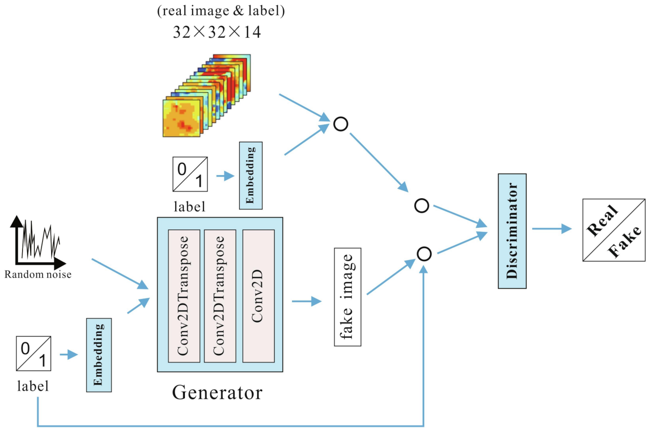
Figure 2.7 Schematic architecture of the cGAN used for data augmentation, showing label embedding, generator structure, and discriminator processing of real and synthetic samples (Wu et al., 2023).
