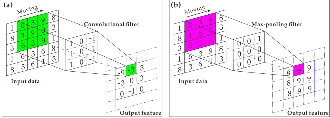
Figure 2.6 Illustrations of (a) convolution and (b) max-pooling operations (Sun et al., 2020).
