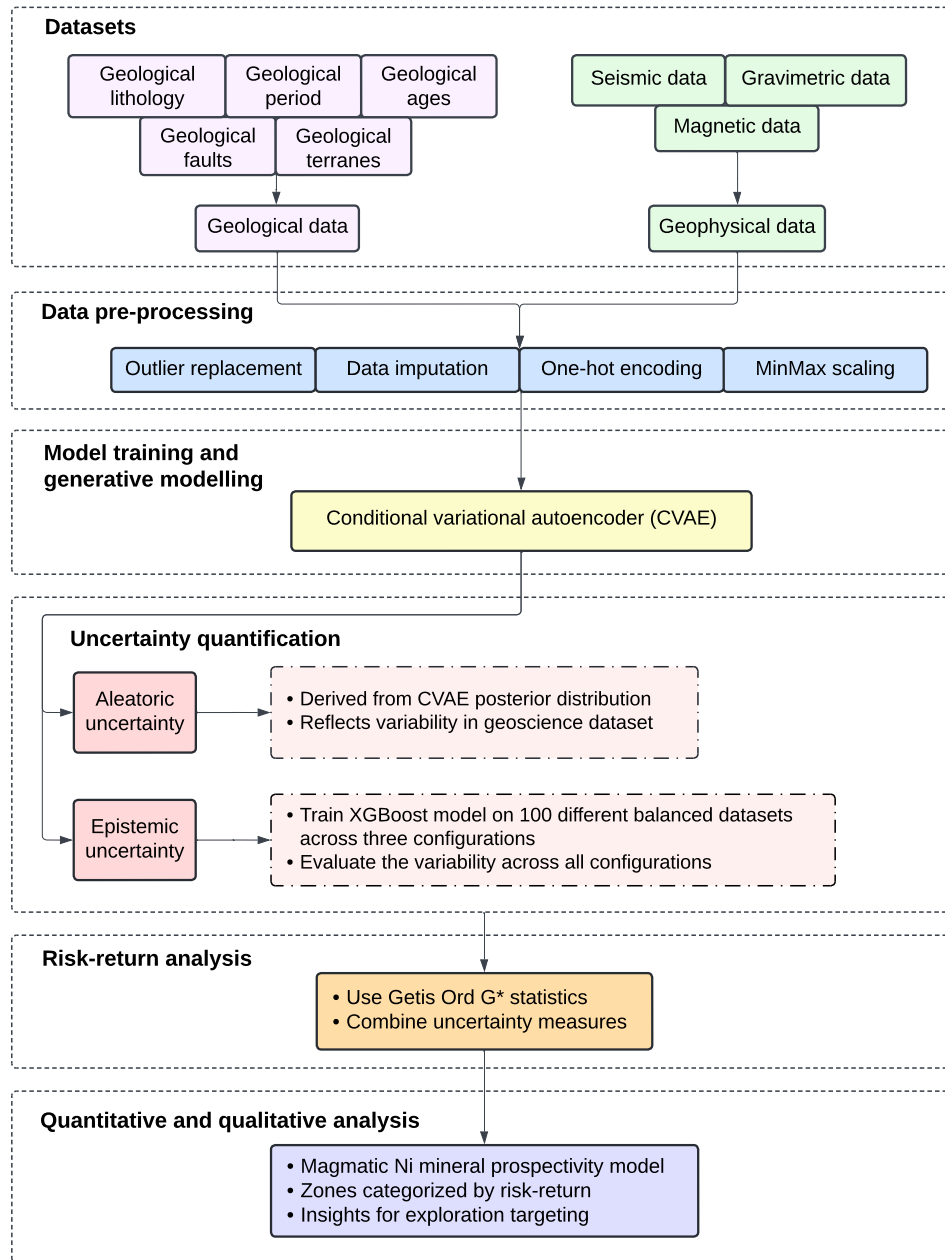
Figure 5.5 Flowchart of key steps involved in the uncertainty and risk-return analysis of prospectivity modelling.
