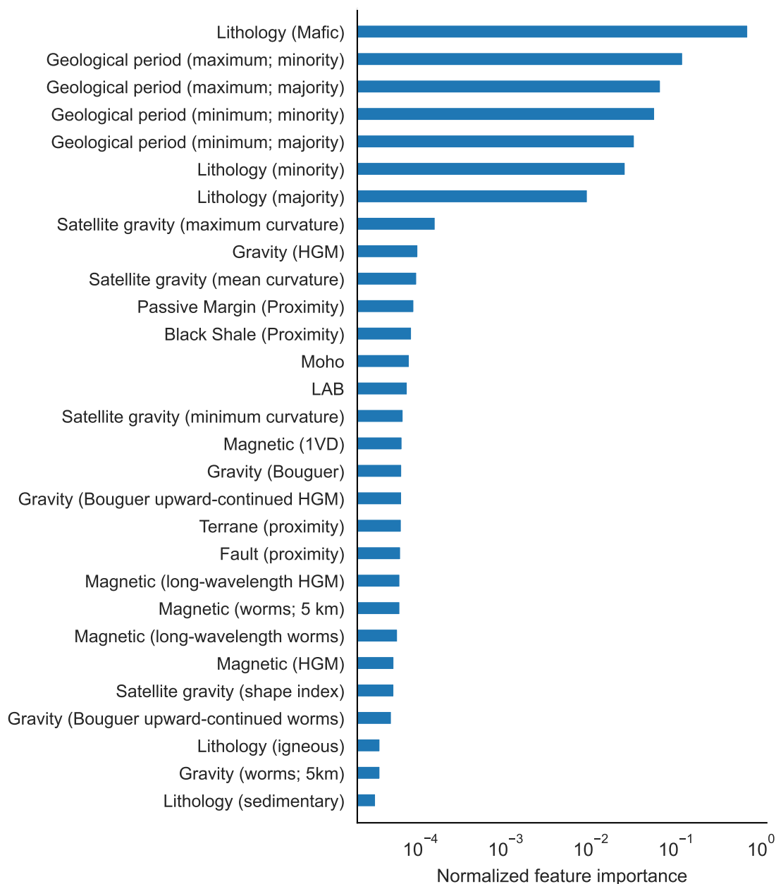
Figure 4.13 Normalized feature importance in the preferred XGBM-CVAE prospectivity model. The importance value of each data set is averaged within its category for one-hot encoded data and directly obtained for non-encoded data. The bars show the average feature importance of each feature, providing insights into their relative significance in the XGBM model's predictions.
