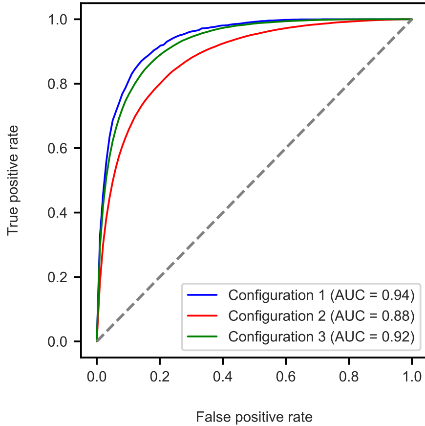
Figure 5.6 ROC curves for the testing dataset that indicate the classification performance of MPMs across three dataset configurations: (1) real geoscience data with CVAE-generated synthetic positive samples, (2) reconstructed data with synthetic positive samples, and (3) a hybrid dataset combining real, reconstructed, and synthetic positive samples.
