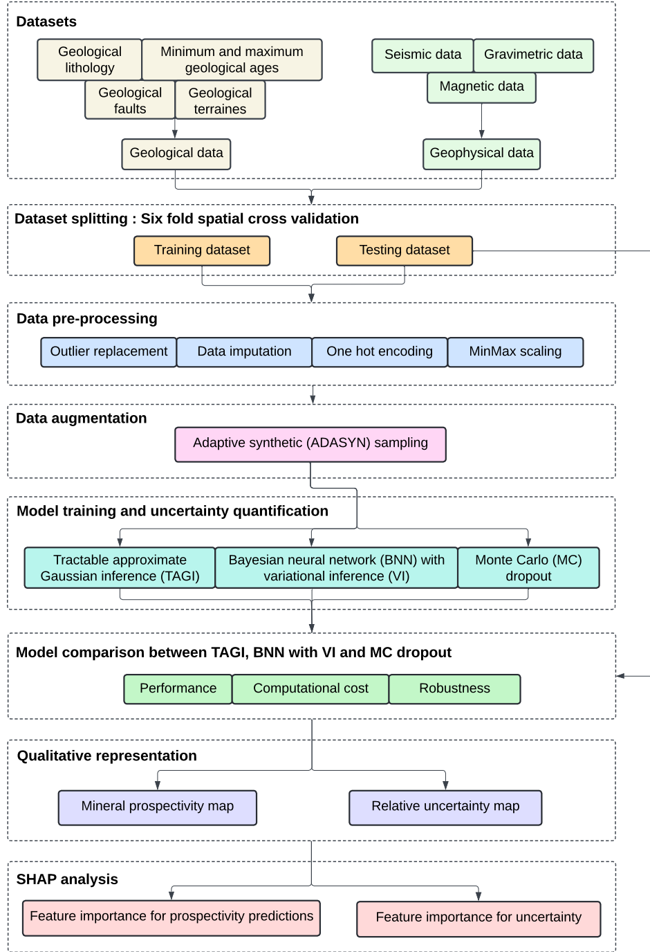
Figure 6.2 Schematic workflow of the proposed MPM framework comparing three Bayesian deep learning methods.
