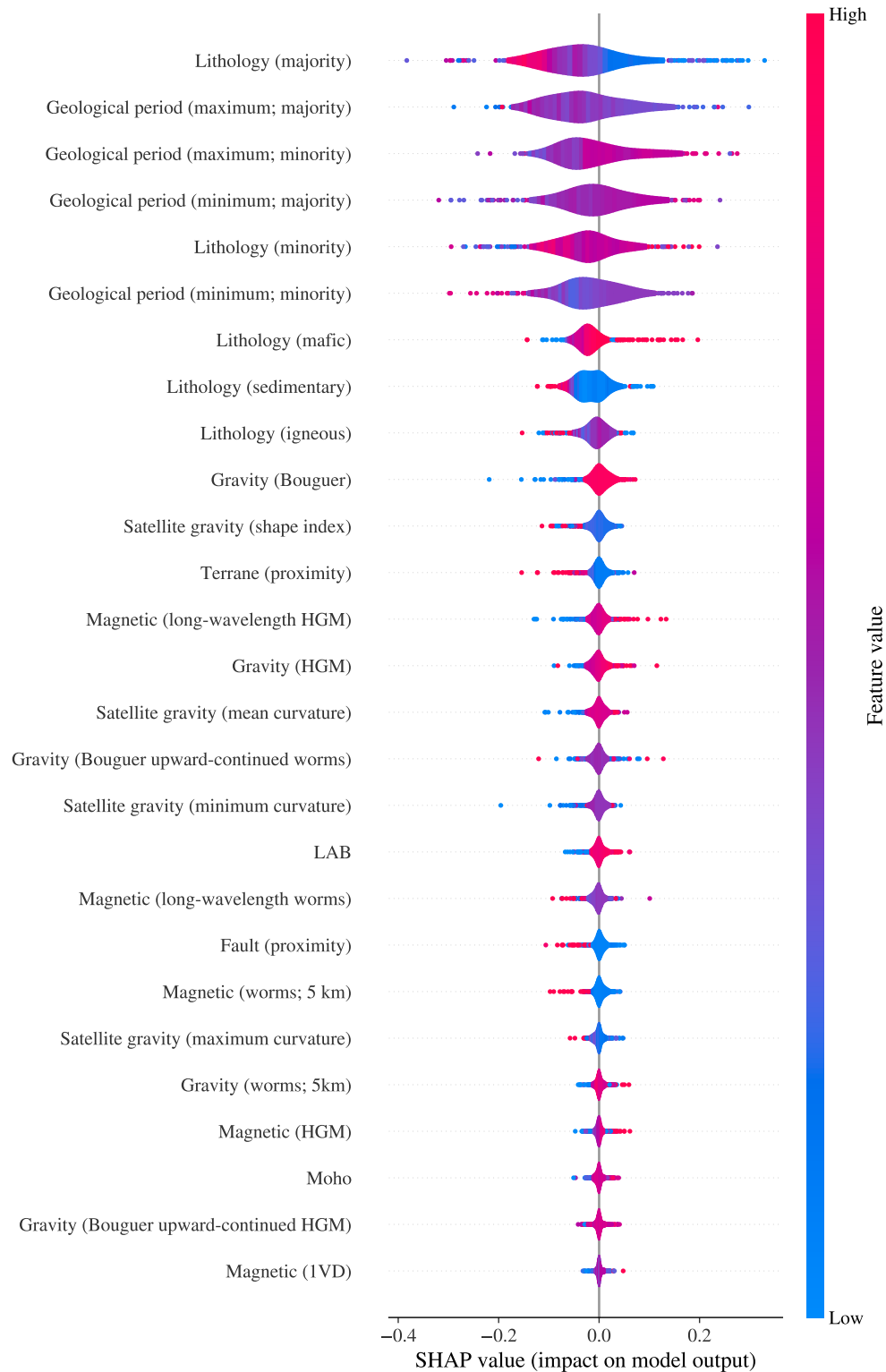
Figure 6.9 SHAP summary plot showing the feature importance for the TAGI model's prospectivity predictions. Each feature's violin shows the distribution of its SHAP values across the test set. The position on the x-axis indicates the impact on the model's output, while the colour represents the feature's value from high (red) to low (blue). The features are ranked from most to least important.
