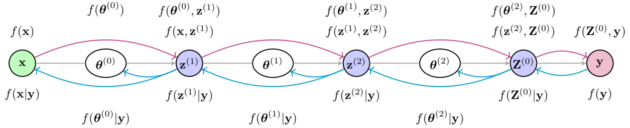
(b) Compact representation of the TAGI model, where \theta = \{\mathbf{W}, \mathbf{B}\} represents the parameters connecting the layers. The forward pass (magenta arrows) propagates uncertainty through the network layers, while the backward pass (cyan arrows) performs layer-wise analytical parameter inference.
