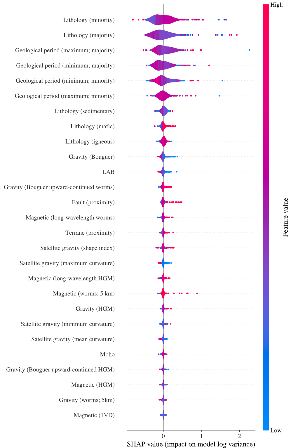
Figure 6.10 SHAP violin plot showing the feature importance for the TAGI model's uncertainty across the test set. The features are ranked by importance, where a positive SHAP value on the x-axis corresponds to an increase in output variance. The colour bar represents the feature's value, with high values shown in red and low values in blue.
