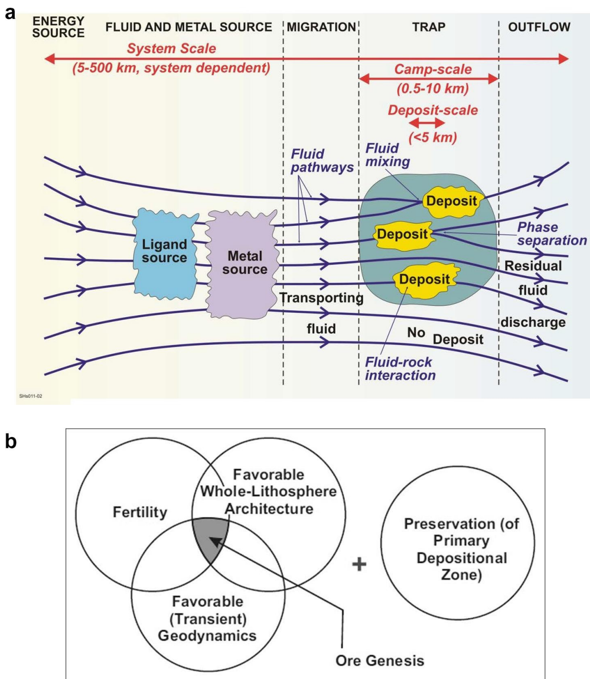
Figure 2.9 Schematic illustrating the difference between two conceptual frameworks for mineral systems. The investigative lens (a) focuses on the causal links between multi-scale component processes (Hronsky and Kreuzer, 2019; Wyborn et al., 1994), whereas the predictive lens (b) highlights the necessary spatial and temporal conjunction of independent elements needed for ore genesis (McCuaig et al., 2010).
