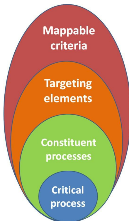
Figure 2.1 A simplified conceptual model of the mineral system, illustrating the translation from the critical process to its constituent processes and targeting elements, and finally to mappable criteria (Yousefi et al., 2019).
