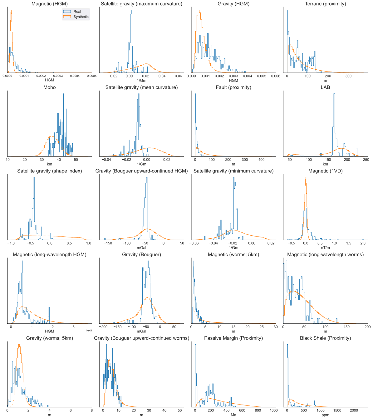
Figure 4.11 Histogram plots of the distributions between generated data from the CVAE model and real geosience data. One hot encoded data subset is deliberately excluded from this figure due to its high dimensionality.
