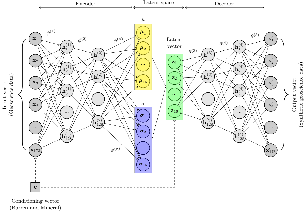
Figure 4.5 The proposed CVAE framework. In the encoder, hidden layers \mathbf{h}^{(l)} are interconnected by linear transformation parameters \phi^{(l)} , whereas in the decoder, they are connected by \theta^{(l)} . The dashed lines represent vector concatenation.
