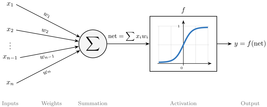
Figure 2.5 Computations performed at a single perceptron unit
