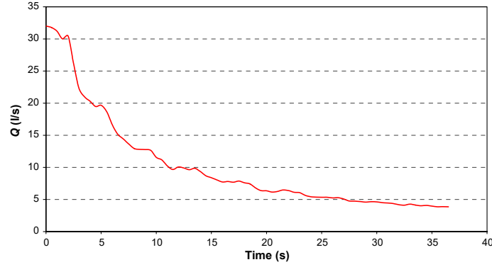
FIGURE 4.26 Hydrographe de Fuamba et al. (2007) [21]
