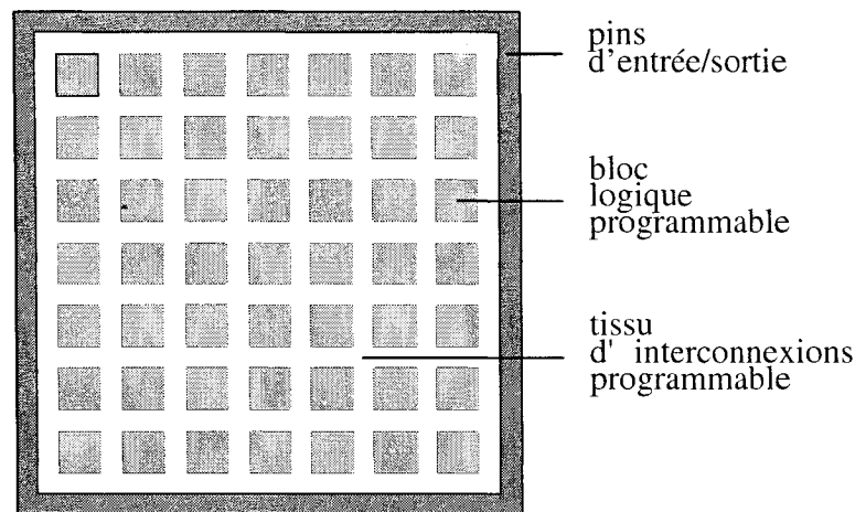
Figure 1.4 Structure d'un FPGA
