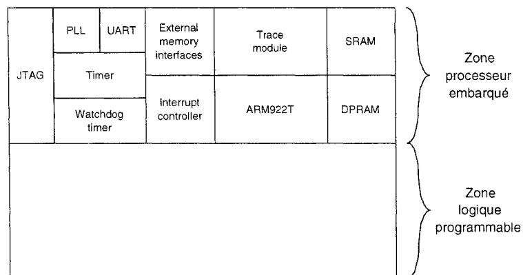
Figure 1.6 Architecture de l'Excalibur
