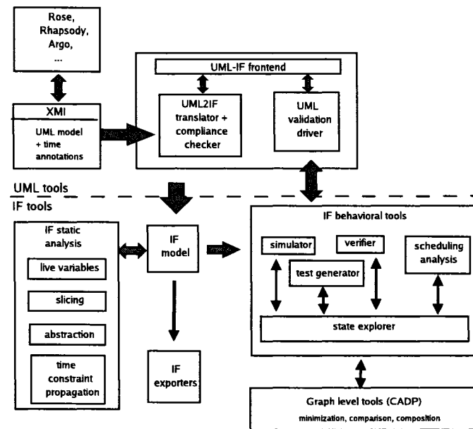
Figure 2.2 Outil IFx
