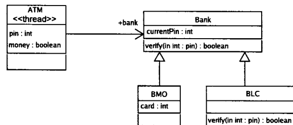
Figure 3.1 Diagramme de classes - ATM
