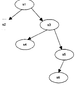
Figure I.1 Graphe
