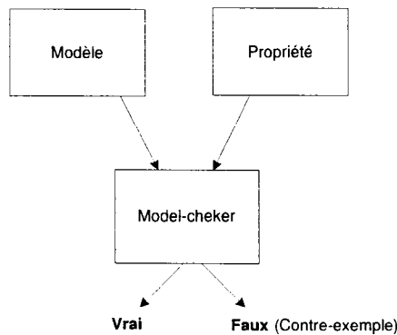
Figure 1.3 Model-checker
