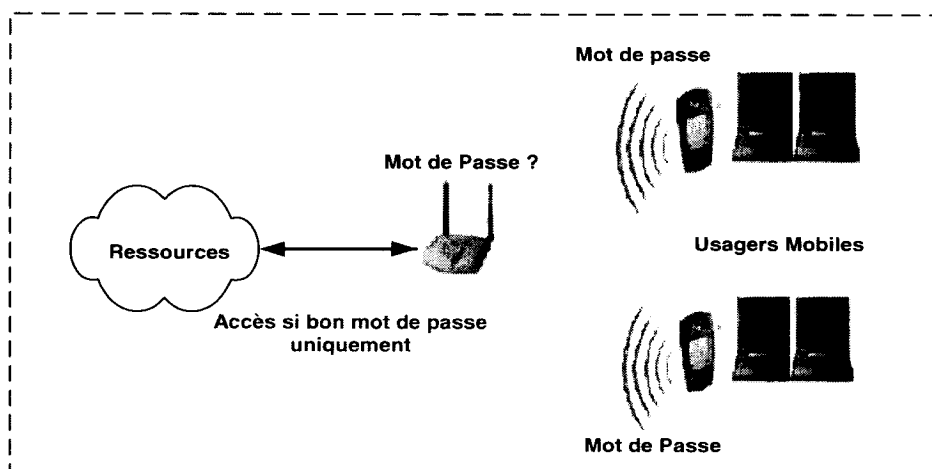
Figure 2.6 Authentification WPA
