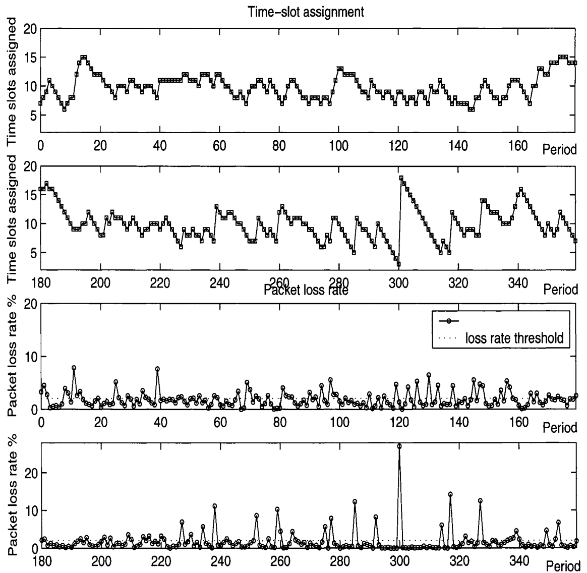
Figure 6.1: Time slots allocation and packet loss rate for case 1-1
