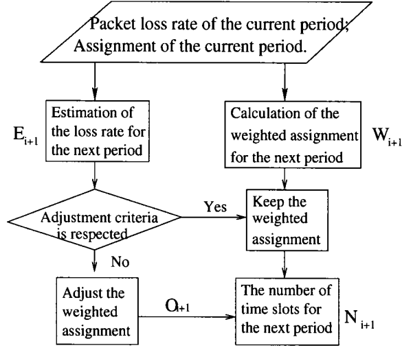
Figure 3.7: The allocation algorithm
