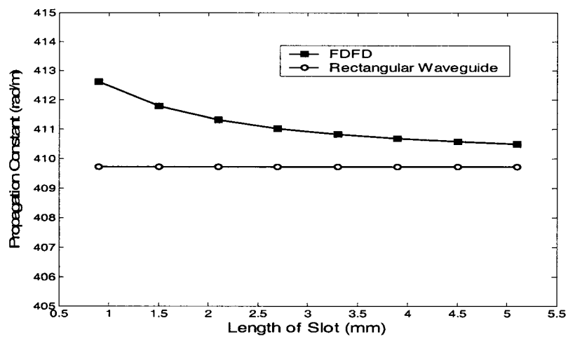
Fig.4.10 propagation constant versus slot length s , when g = 0.6 \text{ mm}
