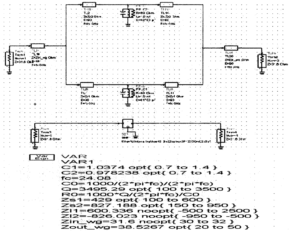
Fig.6.1 Equivalent Circuit Model of Single Cavity Dual-Mode Filter
