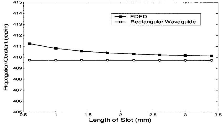
Fig.4.11 propagation constant versus slot length s , when g = 0.4 mm
