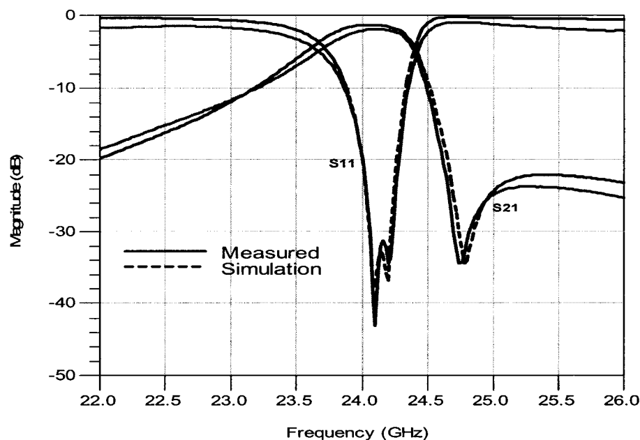
Fig.6.4 Measured and Simulated Frequency Responses with A TZ above the Passband
