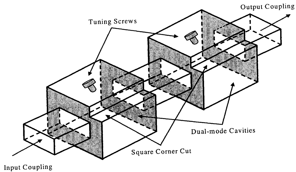
Fig.2.2. Four-Pole Rectangular Waveguide Dual-mode Filter
