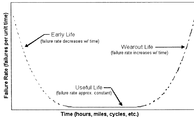
Figure 1.3: An example of a bathtub curve
