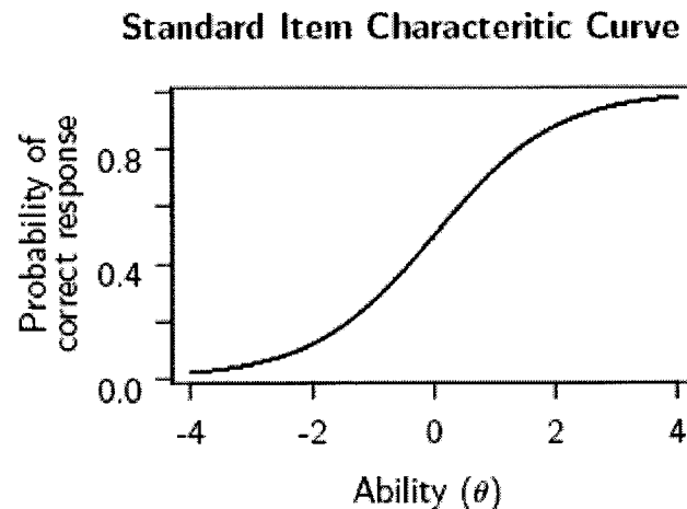
Figure 3-1 Item response curve ( a = 1 , b = 0 , c=0 )
