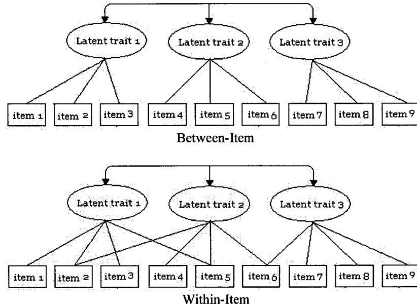
Figure 5-1 Two kinds of multidimensionality
