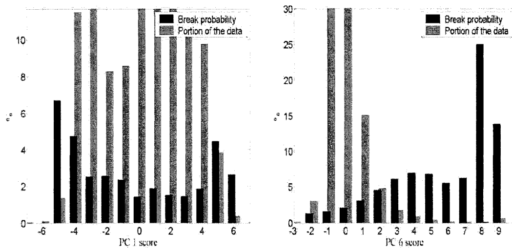
Fig. 5. Observed probability of breaks with respect to the scores of principal components. Left: 1st PC; Right: 6th PC.
