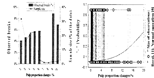
FIG.5. Probability of breaks vs. pulp proportion changes B8; Left: observed; Right: logistic regression prediction model.
