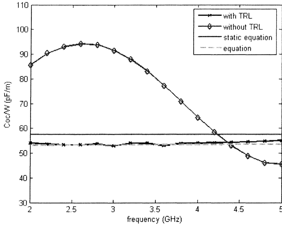
Fig.1.6. TRL-extracted open-end fringing capacitance together with those obtained from the non-TRL parameter extraction scheme and two closed-form design equations [38][39] ( w = h = 0.635\text{mm} , \epsilon_r = 9.9 , L = 10.4\text{ mm} ).
