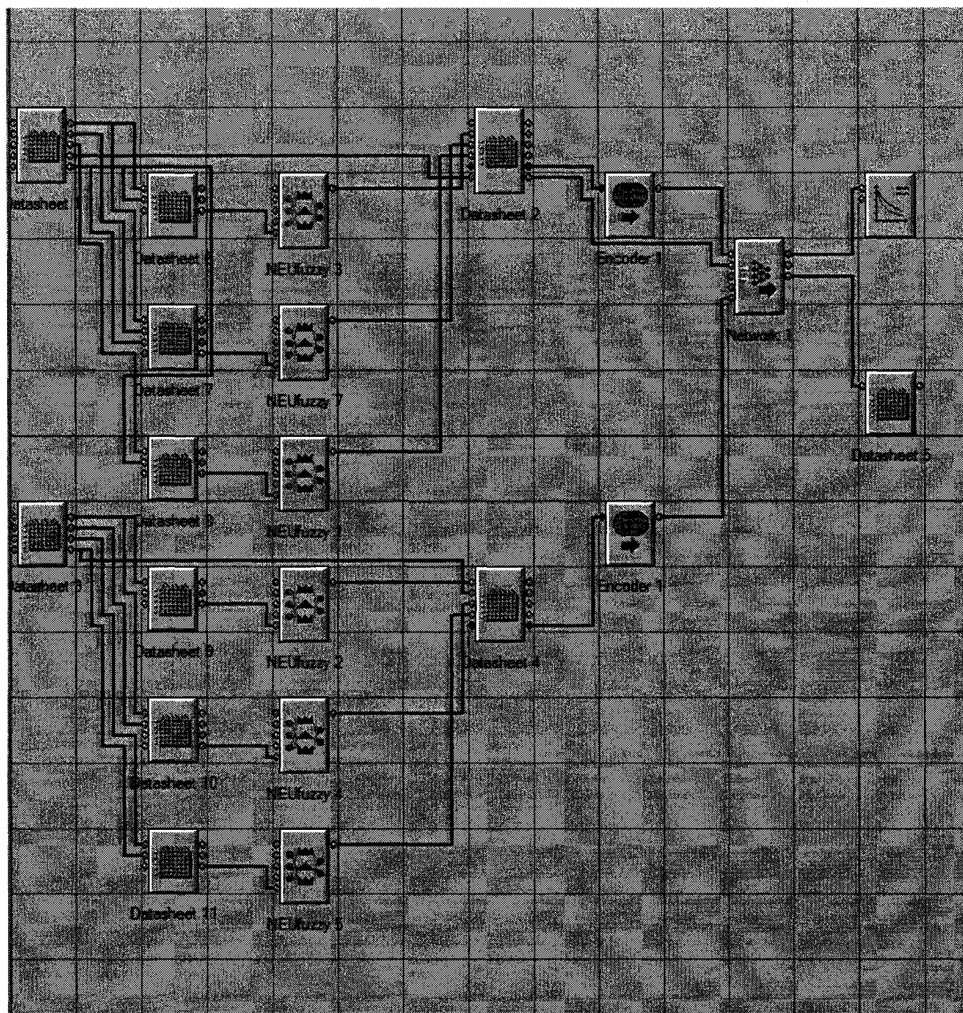
Figure A.3. The NeuFrame Workspace and the Different Connections Between Objects
