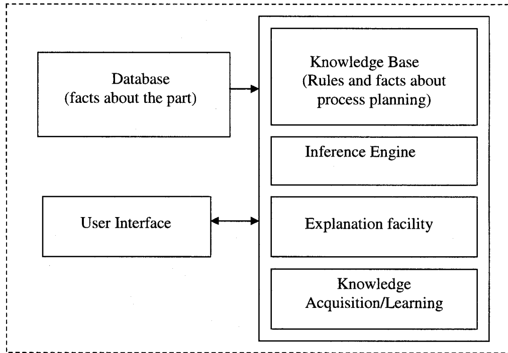
Figure 1.5. Block Diagram of an Expert System
