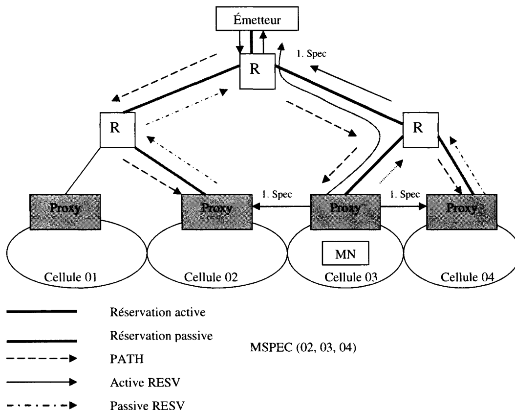
Figure 2.12 Protocole MRSVP
