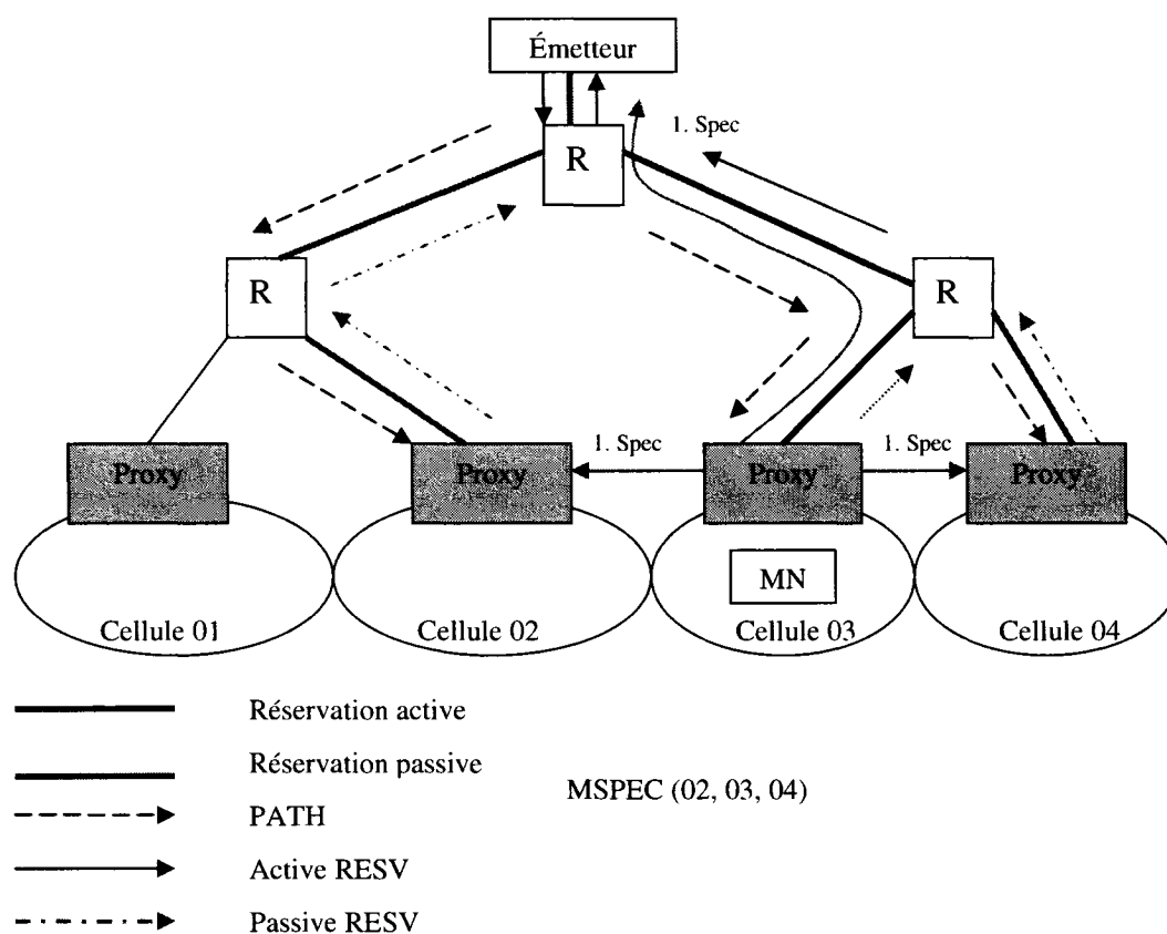
Figure 2.12 Protocole MRSVP
