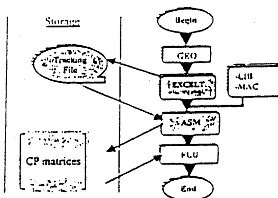
Fig. 1 EXCELT-ASM computational scheme
