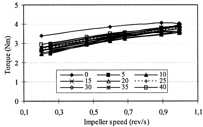
Fig. 5.3.4 Rheological curves of castables with 4 % flake graphite (8.5 % water)
