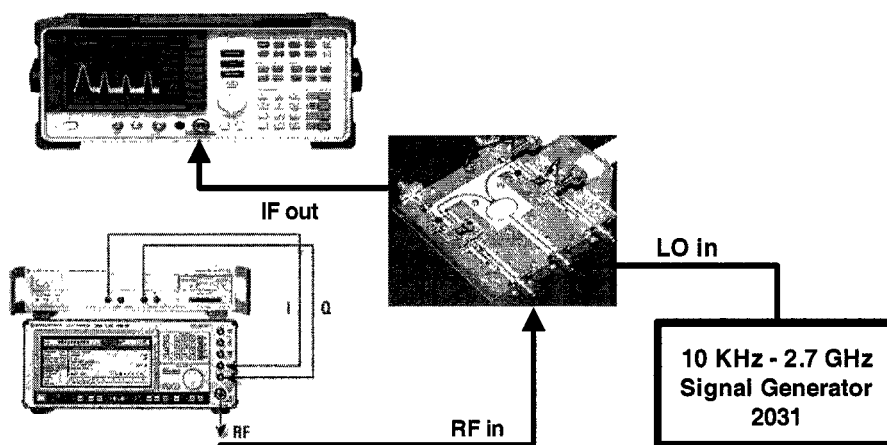
Figure 3- 12 The block diagram of the mixer testing
