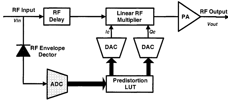
Figure 1- 3 RF/envelope DPD architecture block diagram
