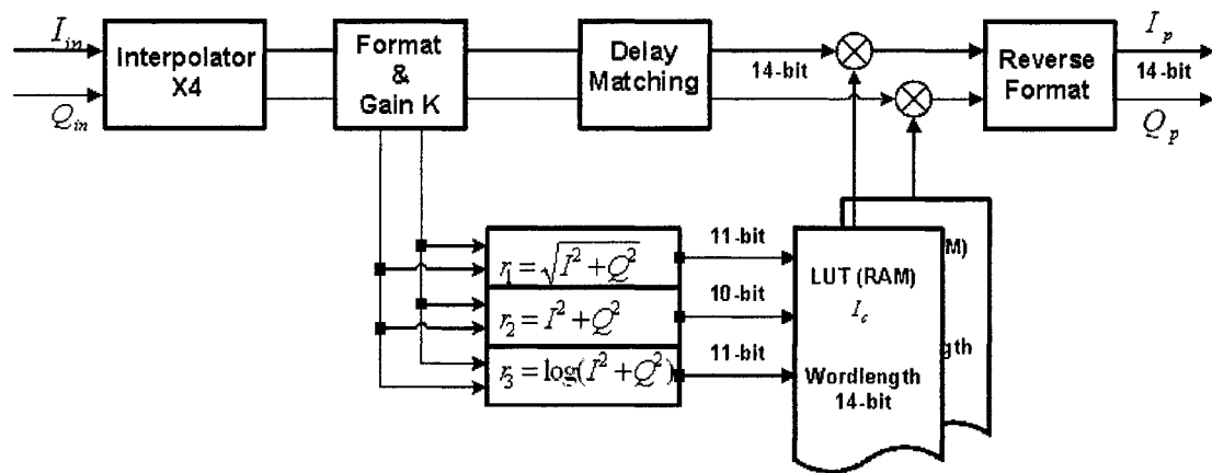
Figure 4- 10 DPD implementation block diagram
