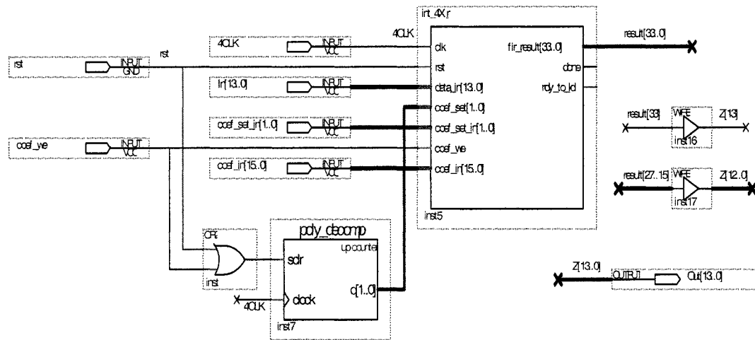
Figure 4- 17 Design of polyphase interpolator
