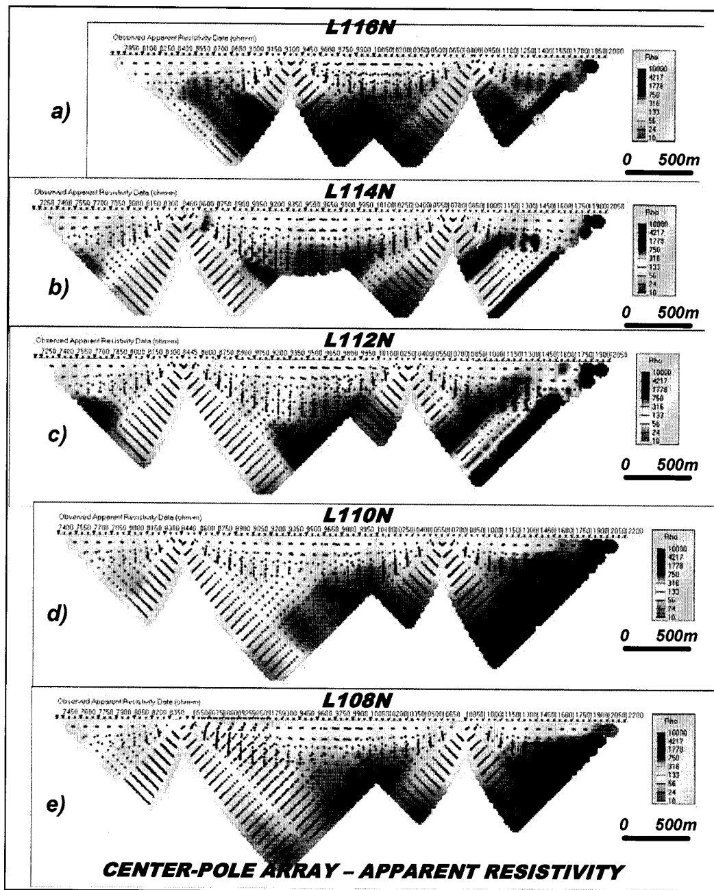
Figure 3.54: Center-pole Array DCIP Apparent Resistivity Pseudosections.
