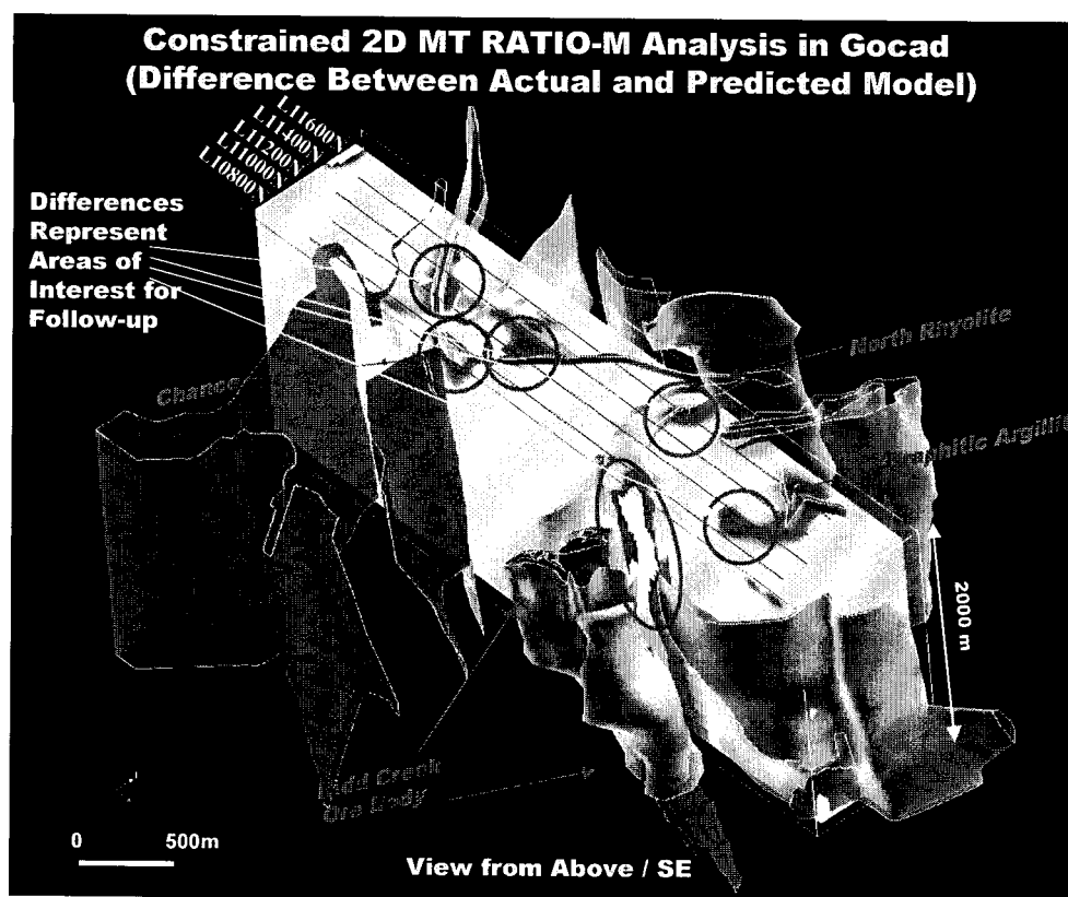
Figure 4.1: Constrained 2D MT Ratio-M Values in 3D Gocad Model.
