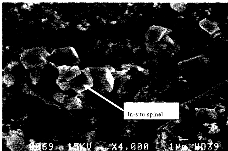
Figure 5.13 SEM microstructure: Formation of in-situ spinel.
