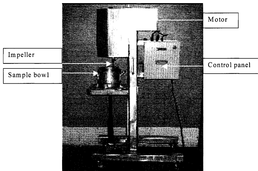
Figure 2.5 IBB Rheometer
