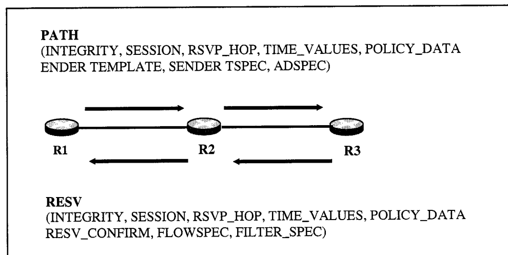
Figure I.1 Session RSVP
