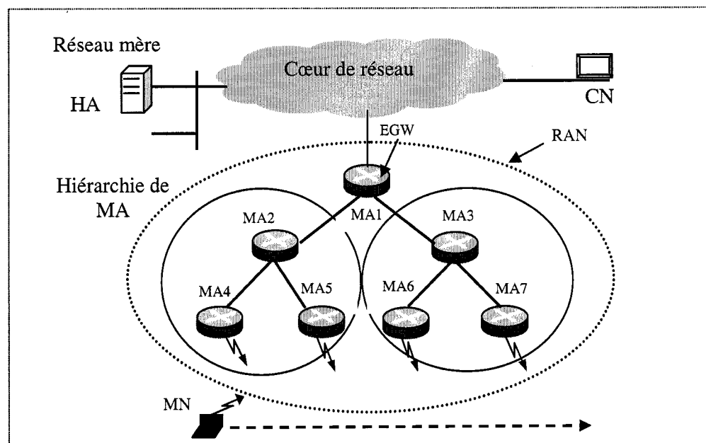
Figure 2.7 Architecture Mobile IPv6 Hiérarchique
