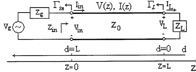
Figure 7.2 Transmission line circuit for mismatched load and generator
