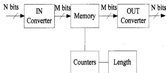
Figure 3.8 Configurable memory-based shift registers
