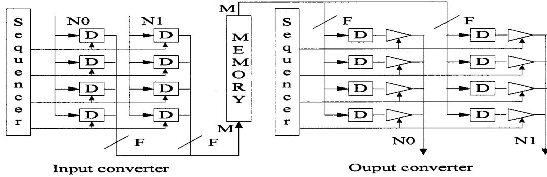
Figure 3.6 Example of a memory based SR with input and output converters
