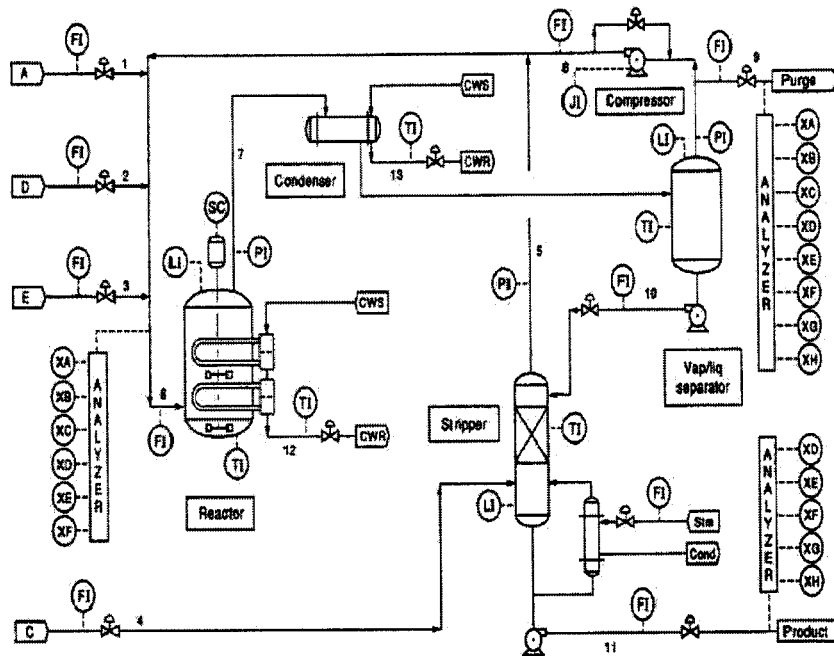
Figure 2.1: Flowsheet of the Tennessee Eastman process (taken from Downs & Vogel, 1993)
