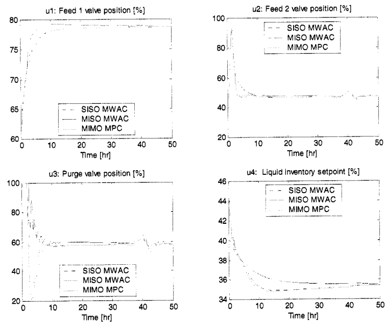
Figure 4.7: Scenario 2 – Manipulated variables – SISO MWAC (dotted black), MISO MWAC (dashed blue) and MIMO MPC (solid green)
