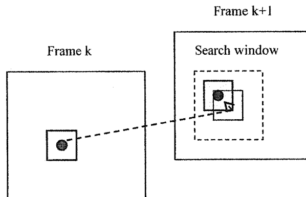
Figure 5.3 Block matching
