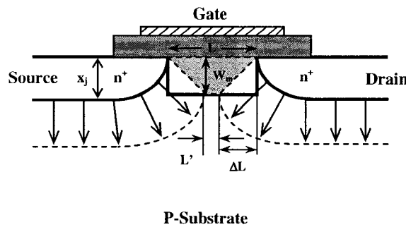
Figure A-8: Threshold voltage-related short-channel effect
