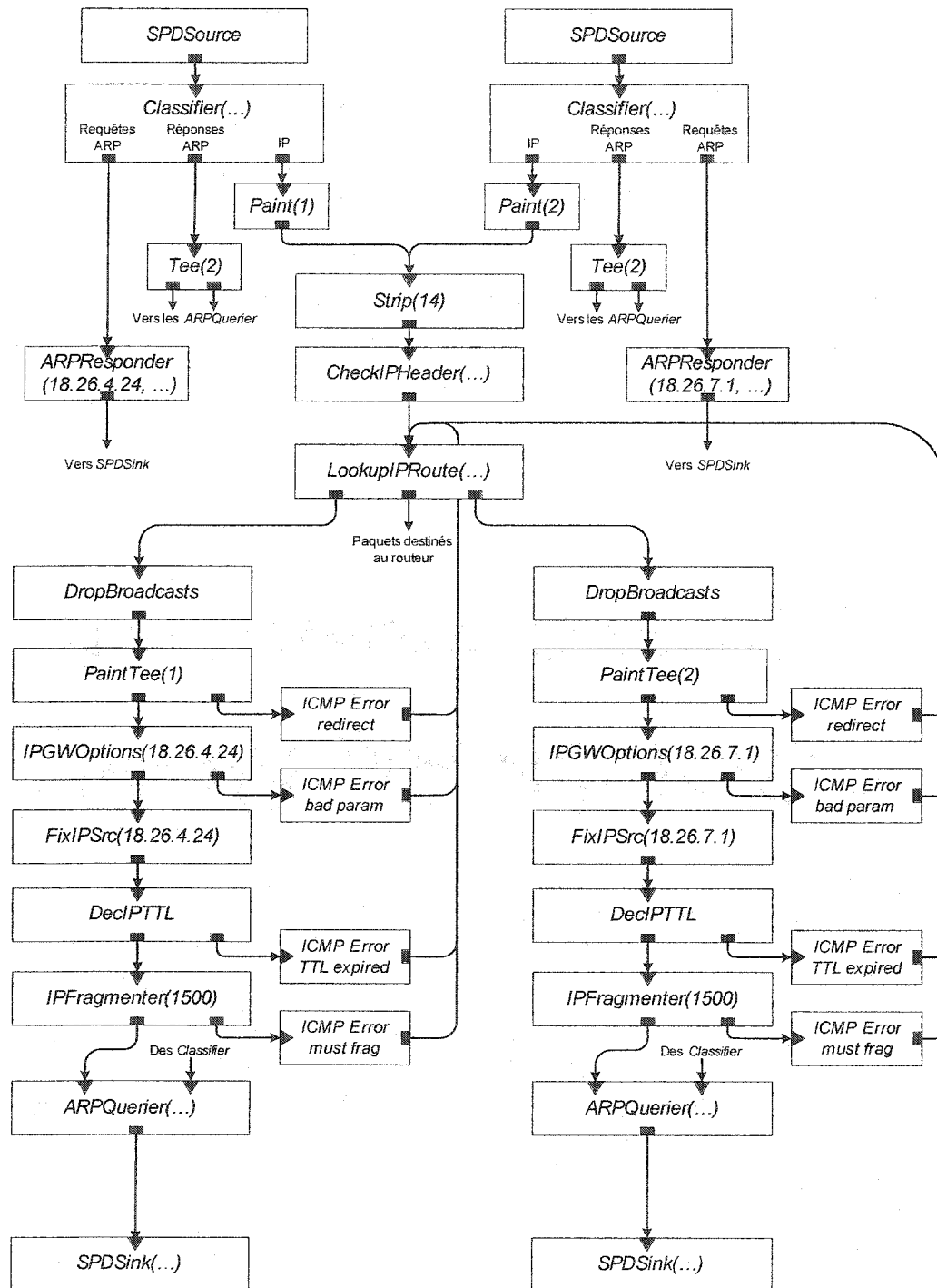
Figure 3.2 : Application IPv4
