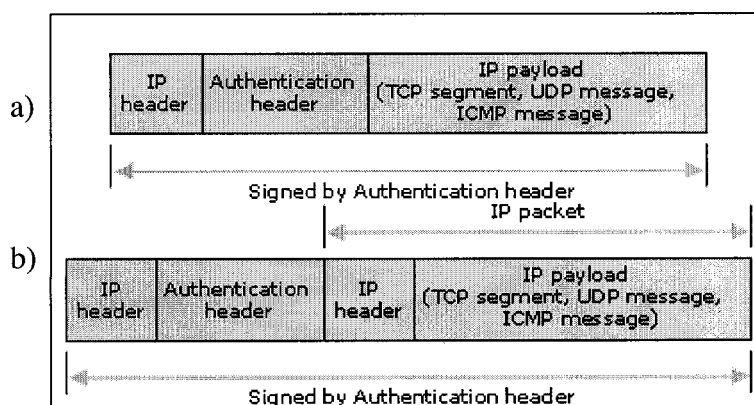
Figure 2.5 Format de paquets AH (a) Mode transport (b) Mode tunnel
