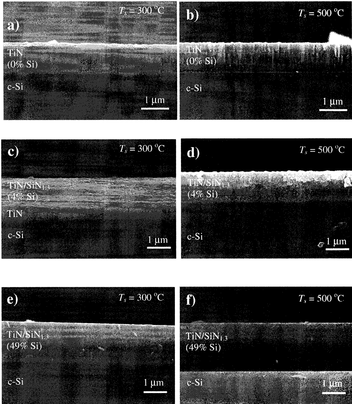
Figure 5.12. SEM cross section micrographs of films deposited at T_s = 300\text{ }^{\circ}\text{C} (a, c, e) and 500\text{ }^{\circ}\text{C} (b, d, f) on c-Si substrate: TiN (a, b), nc-TiN/SiN 1.3 (c, d) with [\text{Si}] = 4\text{ at. } \% , and nc-TiN/SiN 1.3 (e, f) with [\text{Si}] = 49\text{ at. } \%
