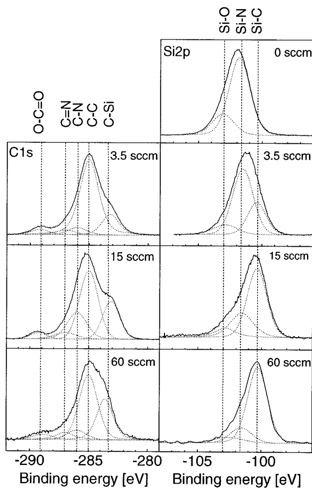
Figure 6.1. High resolution XPS spectra of C 1s and Si 2p core levels for \text{CH}_4 gas flows of 0, 3.5, 15, and 60 sccm.
