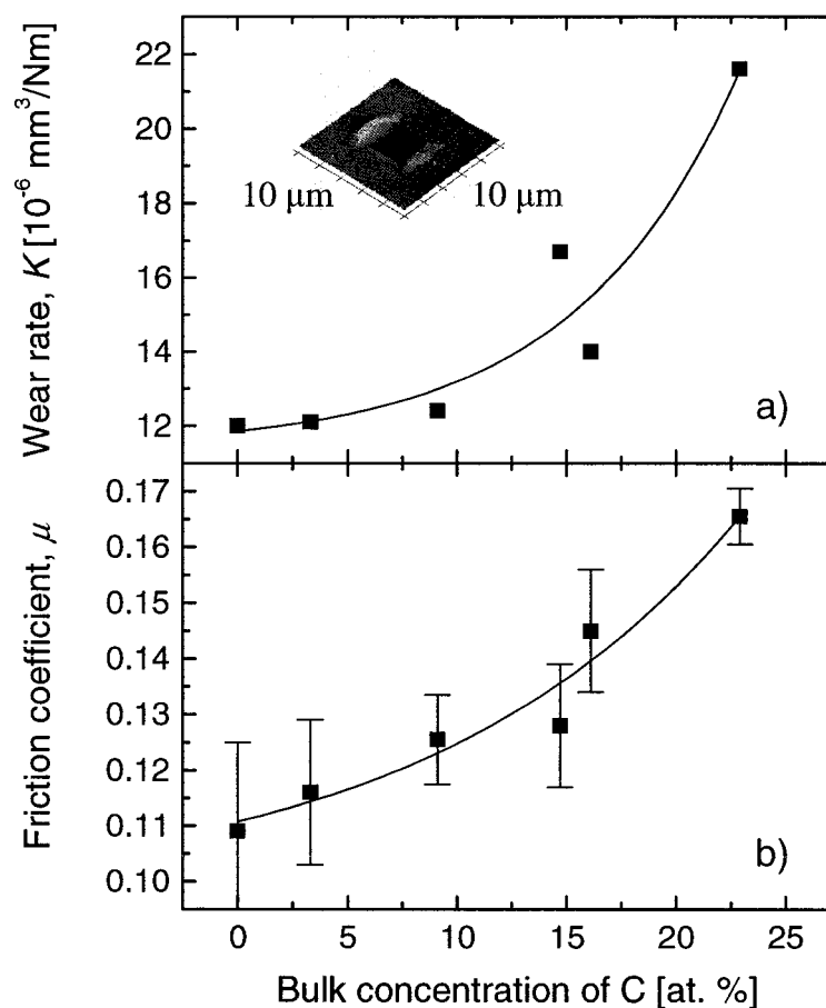
Figure 7.8. The effect of [C_{bulk}] on the wear rate (a) and the friction coefficient (b) for nc-TiC x N y /SiCN films.
