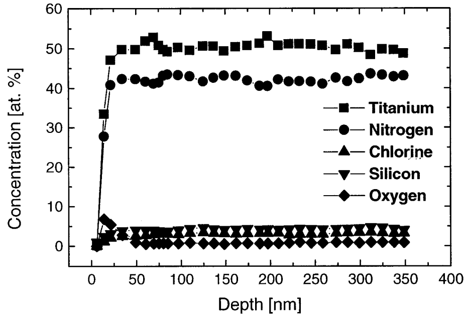
Figure 4.8. ERD TOF concentration depth profile through a nc-TiN/SiN 1.3 film deposited at T_s = 300\text{ }^{\circ}\text{C} .
