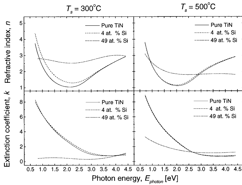
Figure 5.2. The n and k dispersion curves for pure TiN and nc-TiN/Si 1.3 with [\text{Si}] = 4 and 49 at. % fabricated at T_s = 300 and 500^\circ\text{C} .
