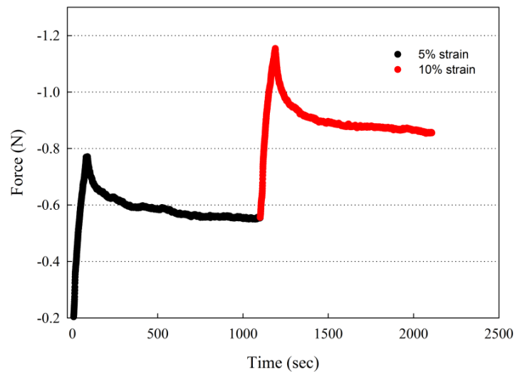
Figure 6-4 : Typical experimental stress relaxation curve of growth plate samples undergoing a two-step semi-confined compression
