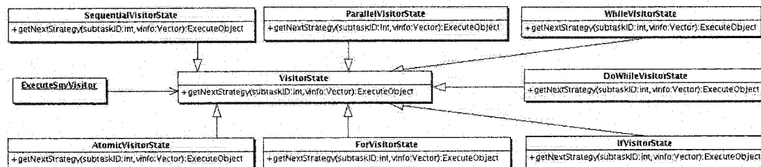
FIGURE 5.19 The classes in the State Pattern
