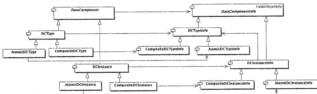
FIGURE 3.2 The DataComponent package UML diagram
