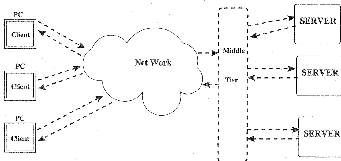
Figure 2.2 Three-tier architecture
