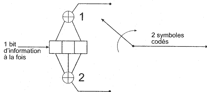
Figure 3.4: Codeur convolutionnel : K = 3, n = 2
