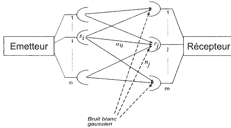
Figure 4.1: Système multi-antennes
