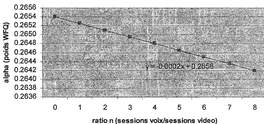
Figure 3.14 Courbe \alpha_{optimal}=f(n)
