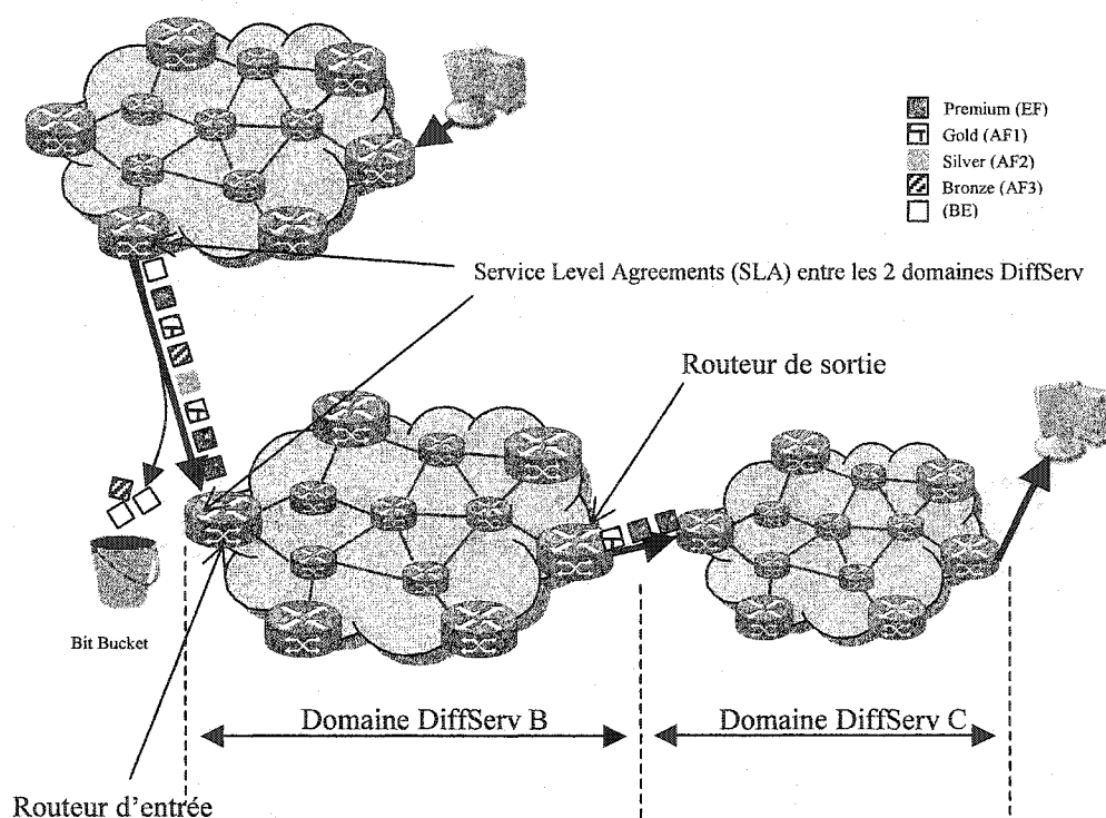
Figure 2.5 Modèle architectural de DiffServ
