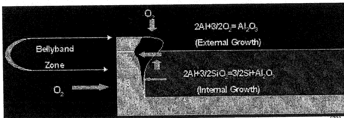
Figure 1.2: Three Zones in Aluminium Treatment Furnace Lining, according to Allaire [72]
