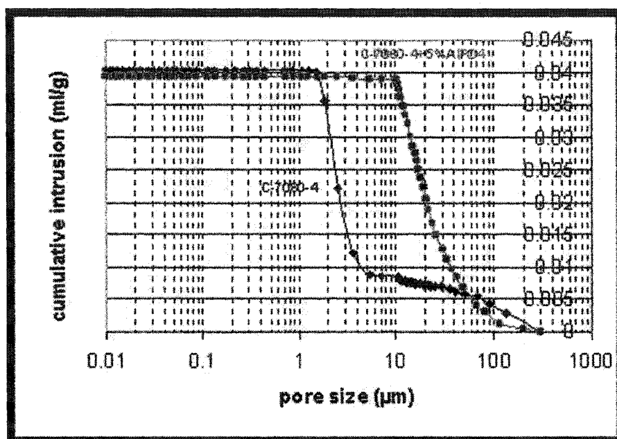
(a) Cumulative Intrusion vs. Pore Size
