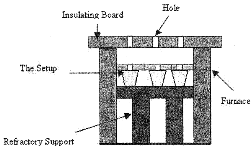
Figure 2.3: Top-Open -Furnace Set-up
