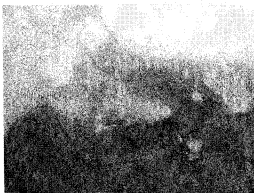
Figure 3.1.25: C-7080-4+5%BN Refractory corroded by corundum Molten Al penetrates through re-ox reaction corundum, and stops at a pore. Bottom: re-ox reaction corundum; Middle: direct oxidized corundum(black) ×500
