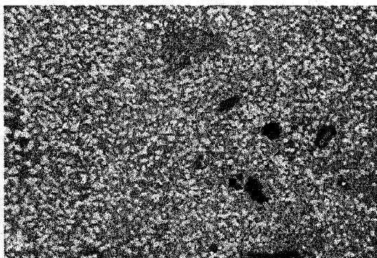
Figure 3.1.31: C-7080-4+5%AlPO 4 Ox-Re Reaction Corundum Area ×50
