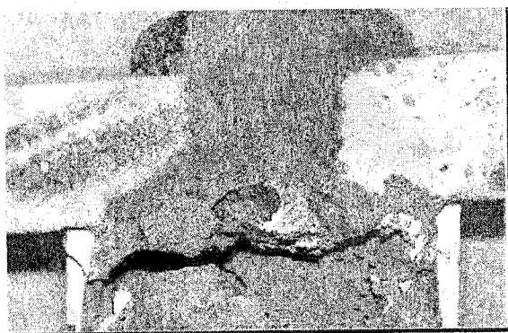
Figure 2.12: 22# C-7080-4+5%CAS, after1286°C×29h,7075 alloy
