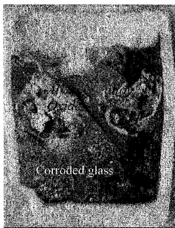
Figure 4.1: Corrosion aspect of W-glass (window glass).
