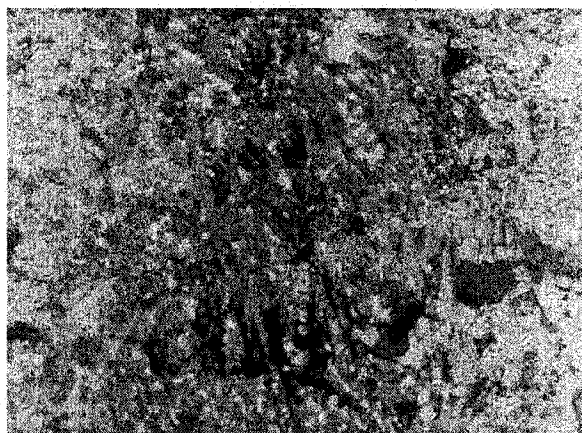
Figure 3.2.9: C-7080-4+5%BaCO 3 Corroded Area ×50
