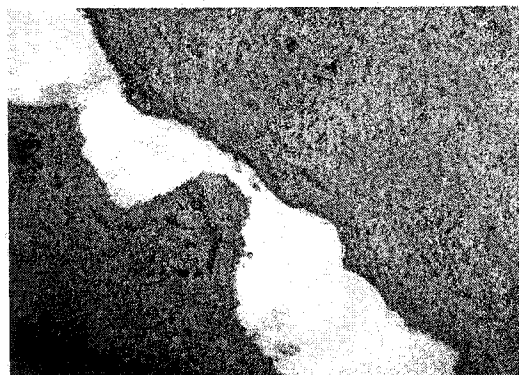
Figure 3.1.19 : C-7080-4+5%CaB 6 Molten Al goes through corundum \times 10
