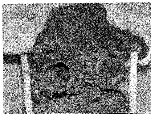
Figure 2.15: C-7080-4+5%Talc, after(1214-1243°C)×72h,7075 alloy
