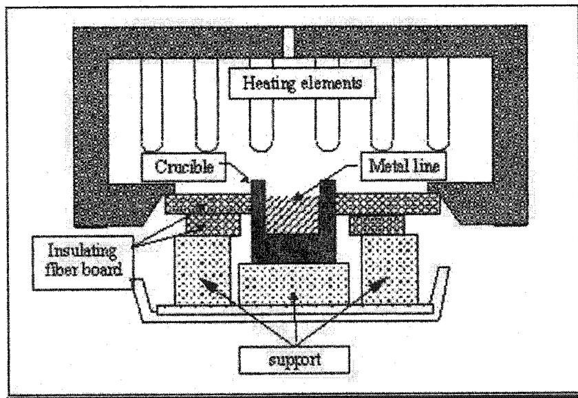
Figure 1.5: CIREF Bellyband Test Set-up [72]
