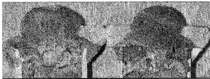
Figure 2.5: left: 66# C-7080-4+5%SiC, AMZ, (1212-1222)°C × 37 h, loose sealing, bottom-open-furnace; right: 111# C-7080-4+5%SiC AMZ, 1200°C × 40h, top-open-furnace
