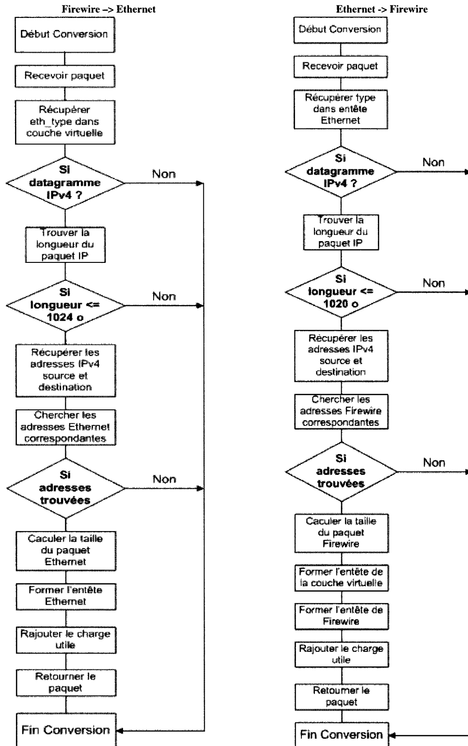
Figure 3-11. Organigramme de la conversion Firewire - Ethernet
