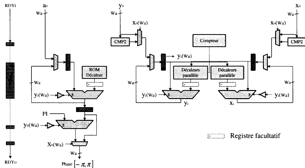
Figure 5.10 – CORDIC
