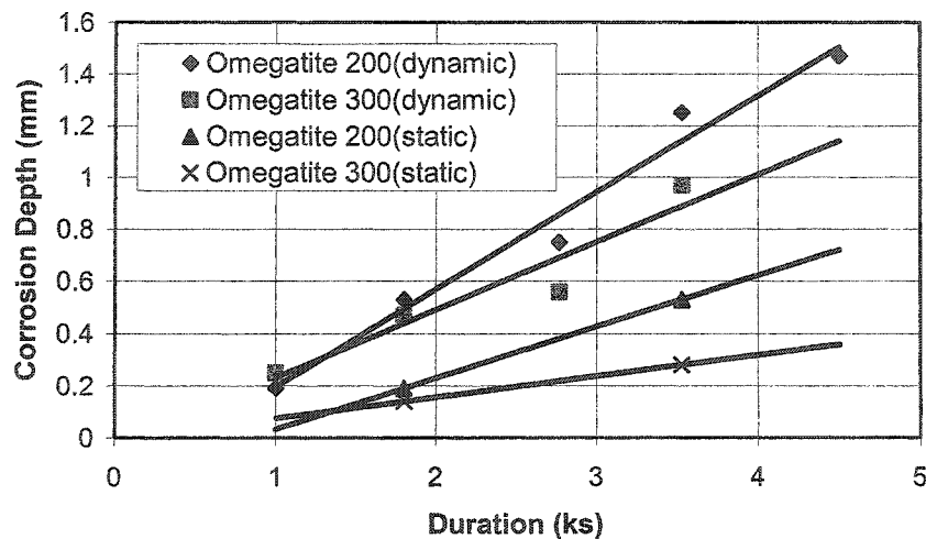
Fig.2-23 Difference between dynamic corrosion and static corrosion [14]
