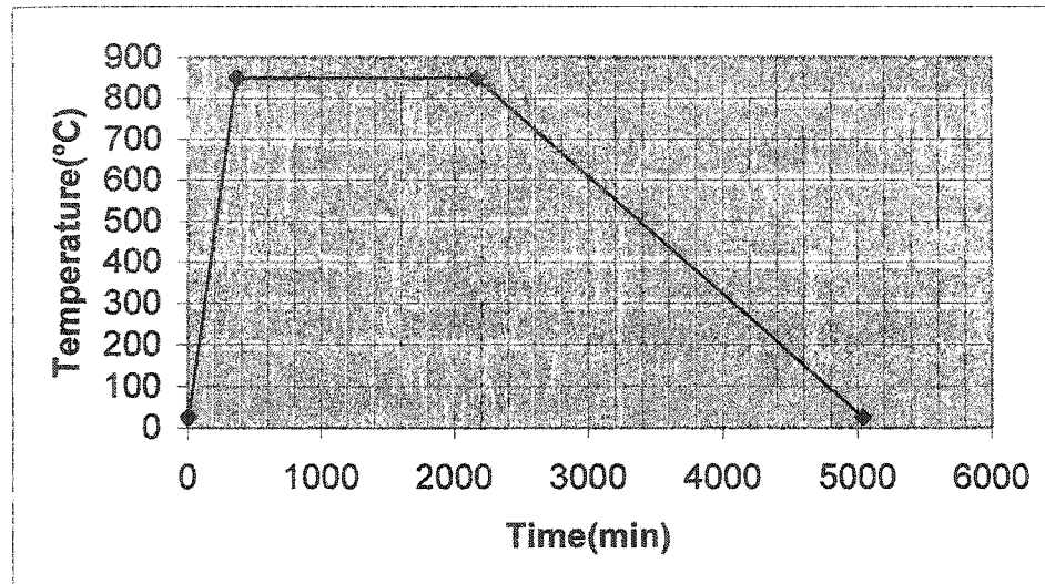
Fig.3-9 Operating curve of the furnace during test
