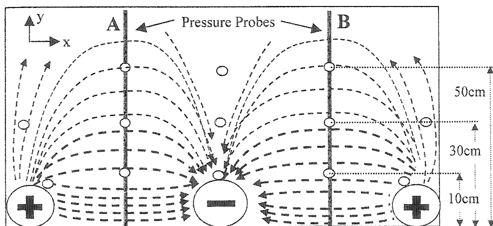
Figure 7.10: Flow Line Pattern in the “+ - +” Configuration
