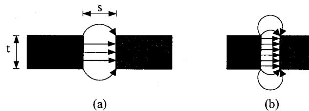
Figure 3.17: Effect of scaling on lateral flux capacitors: (a) before scaling and (b) after scaling.
