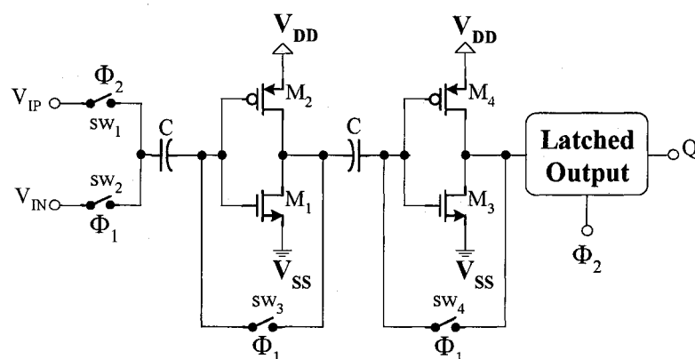
Figure 5.12: Low-Voltage high-speed autozeroed comparator.
