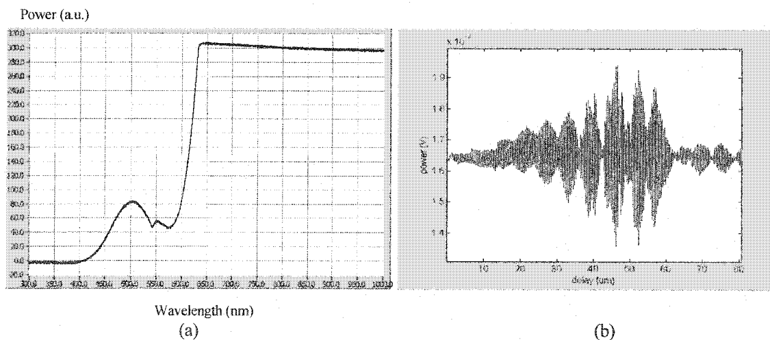
Figure 7.6 Spectrum and interference signal of a halogen lamp
