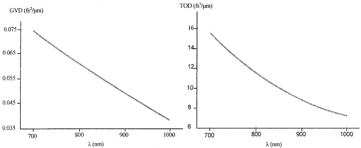
Figure 3.3 The Ti:Sapphire GVD and TOD as a function of the wavelength [8]
