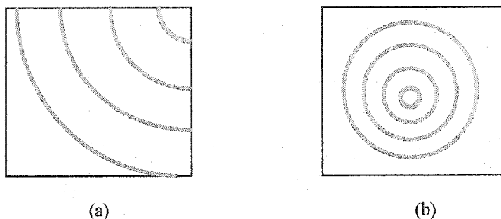
Figure D-1 The interference fringes
