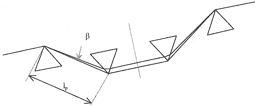
Figure 3.4 Position of the prism pair
