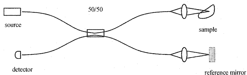
(a). Fiber-optic interferometer
