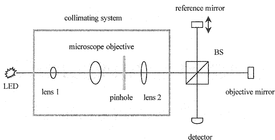
Figure 7.3 Schematic diagram of the white LED Michelson interferometer
