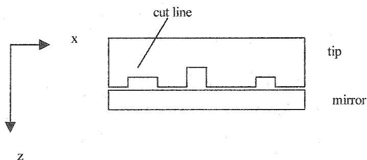
Figure 7.16 Structure of the first sample
