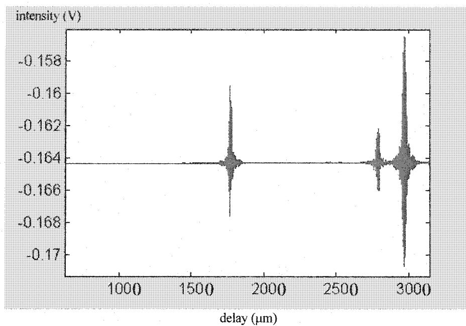
Figure 6.6 An interference signal of three layer sample
