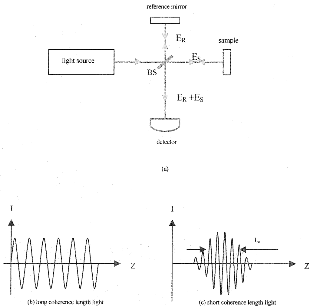
Figure 1.1 A schematic diagram of a standard OCT setup
