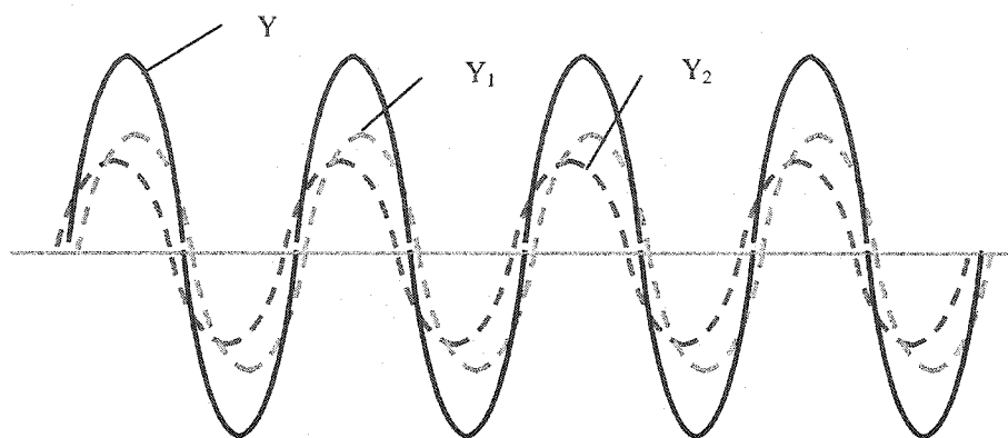
Figure 4.3 Superposition of two harmonic waves Y_1 and Y_2
