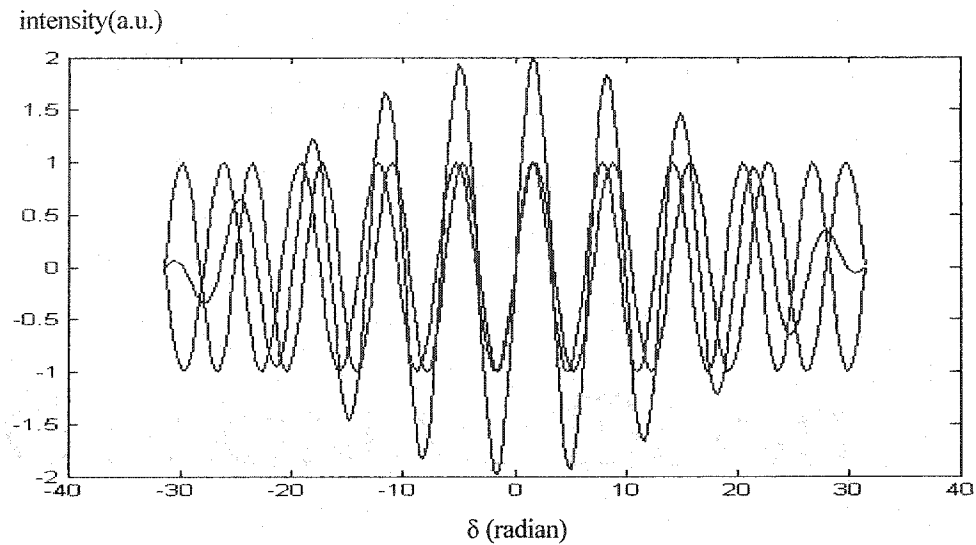
Figure 4.6 The interference pattern of two waves
