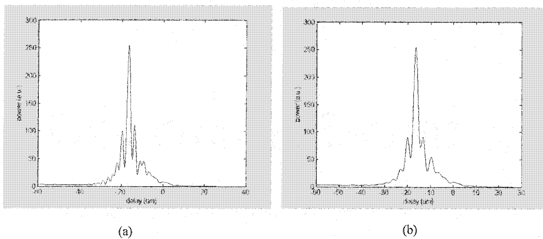
Figure 7.5 The envelop of the interference signal after filtering and cutoff
