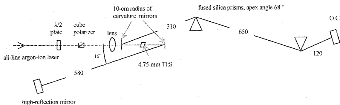
Figure 3.1 The schematic diagram of the Ti:Sapphire laser cavity. The lengths are in mm
