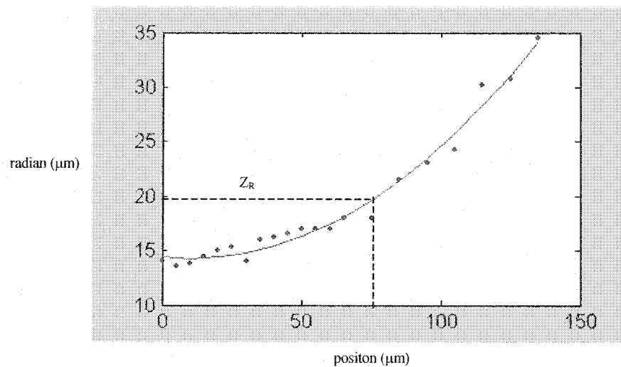
Figure 7.14 Final shape of the focusing beam – The center of the beam is given by the horizontal axis
