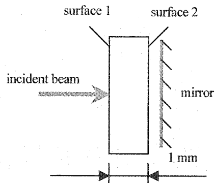
Figure 6.5 The three layer sample
