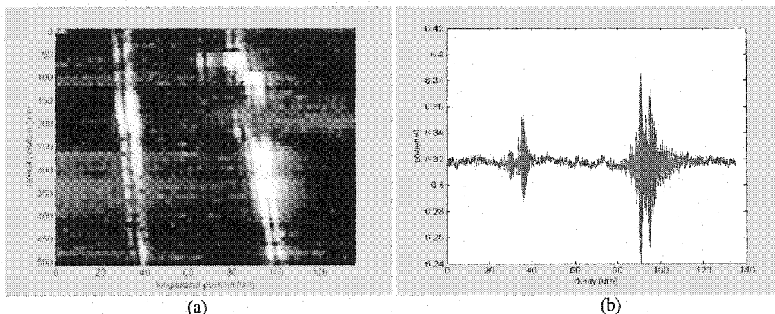
Figure 7.17 Results of the OCT scanning of the first sample
