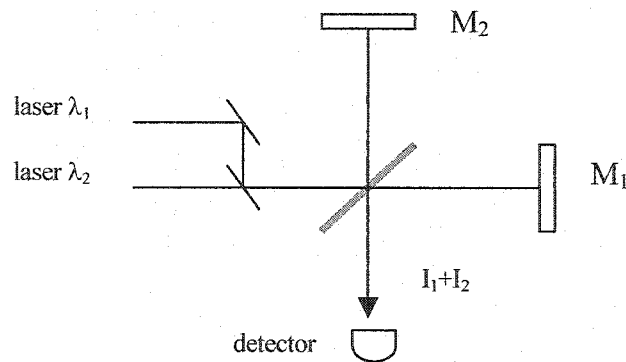
Figure 4.5 Interference between two lights with different wavelengths
