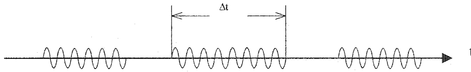
Figure 4.4 A wave consists of wave trains
