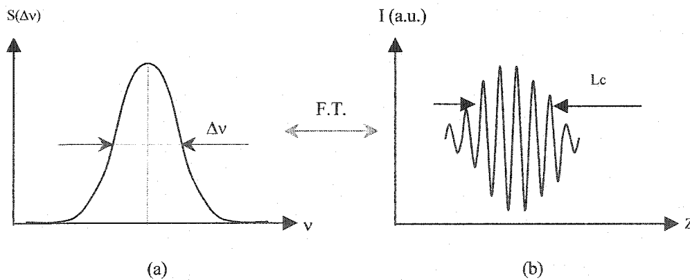
Figure 4.8 The Fourier transformation (F.T.) relationship between the spectral density of a continuous spectrum source and the interference trace
