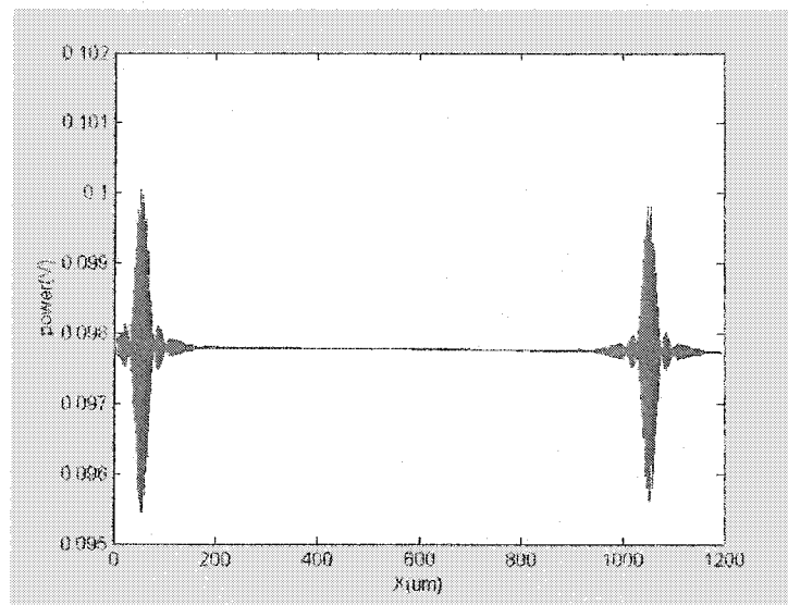
Figure 6.3 An interference signal produced by a longitudinal scan
