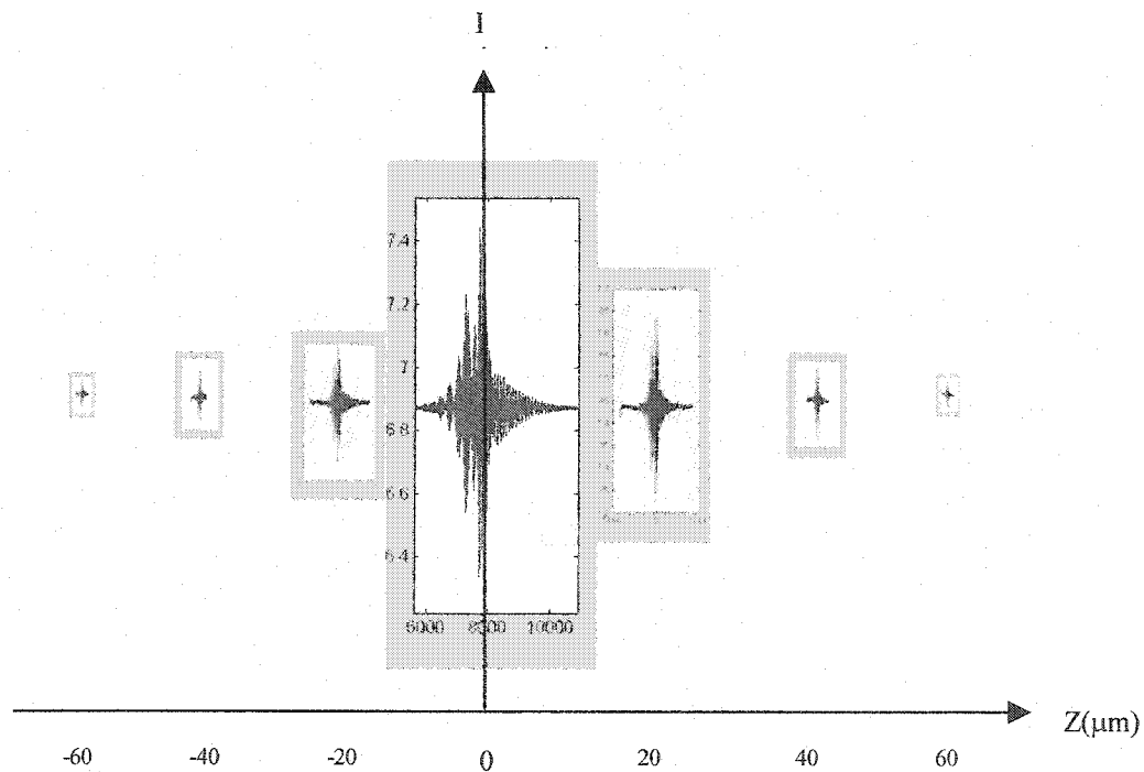
Figure 7.15 Real scanning range of the OCT setup
