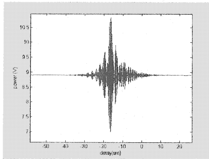
Figure 7.4 Recorded basic interference signal of the white LED source
