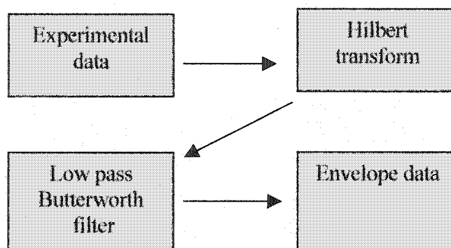
Figure 5.3 Block diagram of the final data processing system
