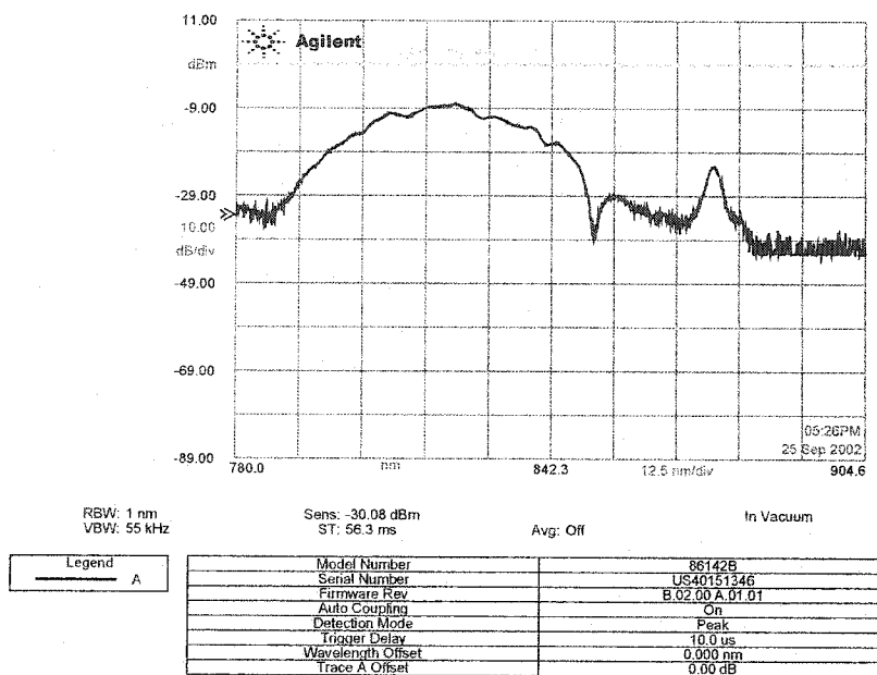
Figure B-1 The spectrum of the ultra-short pulse laser
