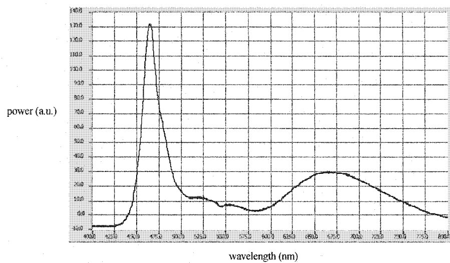
Figure 7.2 Spectrum bandwidth of white LED
