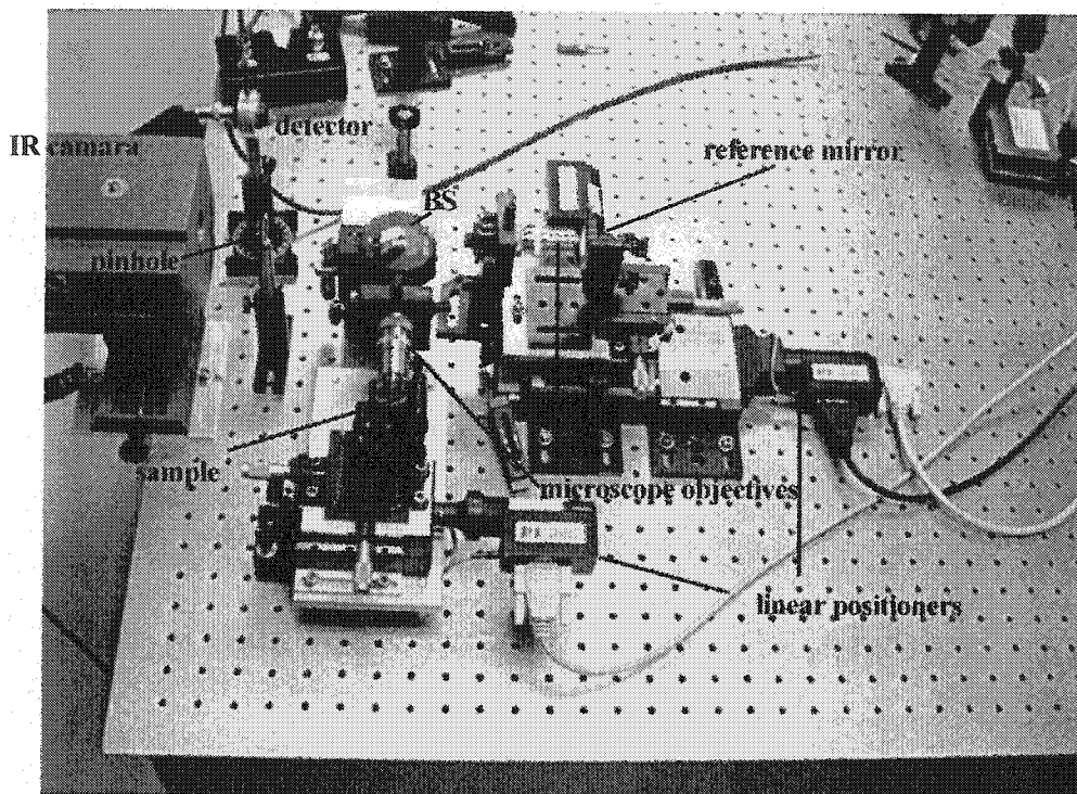
Figure 7.7 Experimental setup of the OCT with white LED
