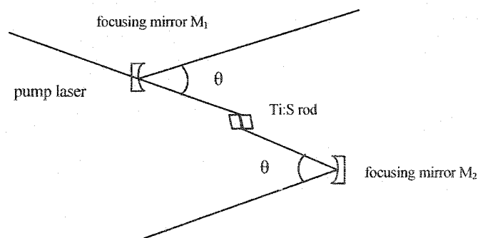
Figure 3.2 The main parts of the laser cavity
