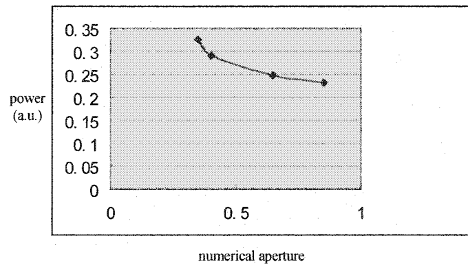
Figure 7.11 The focal spot intensity vs the NA value of the microscope objective
