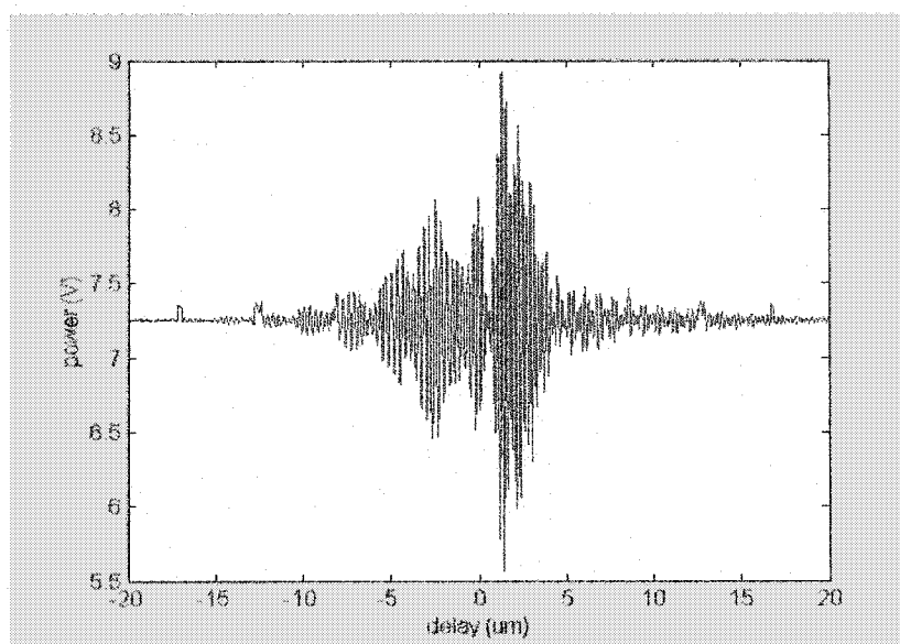
Figure 7.9 Interference signal detected after putting two microscope objectives in position
