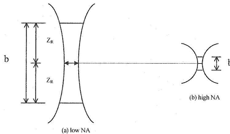
Figure 1.2 A focusing beam shape by low and high numerical aperture (NA)
