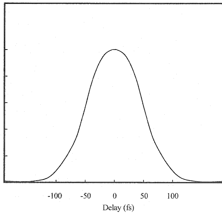
Figure C-2 The autocorrelation trace of ultra-short pulse laser
