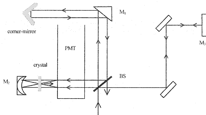
Figure C-1 The optical schematic of the FR-103 autocorrelator
