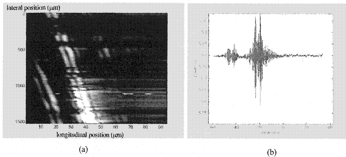
Figure 7.21 Experimental results of the mica sample by the white LED source
