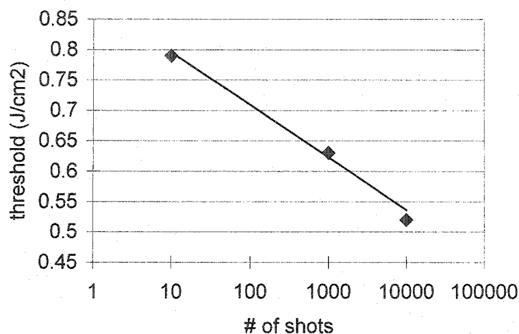
Figure 8.4 Ablation threshold decreases with number of shots [30]
