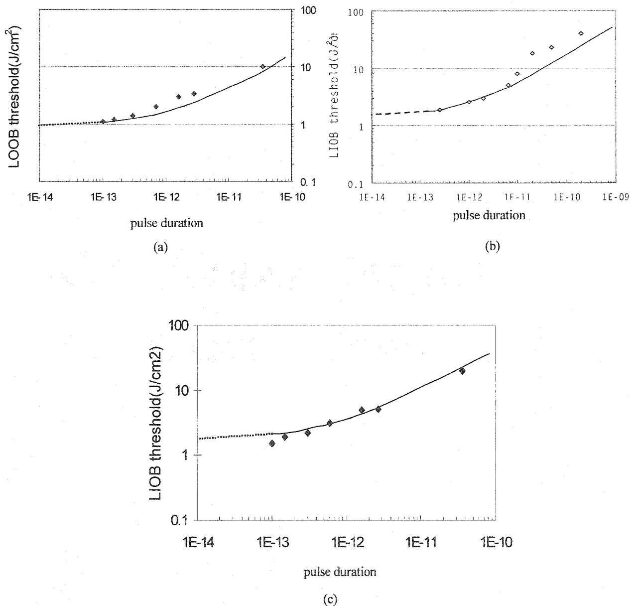
Figure 8.3 The threshold of LIOB as a function of pulse duration on human enamel, human corneal tissue, and bovine brain tissue
