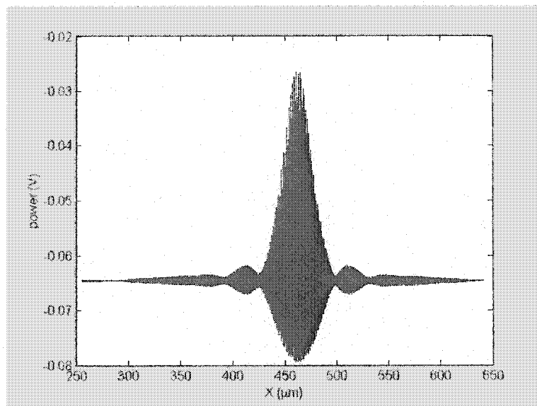
Figure 2.4 The interferometric trace received for the quality test of the OCT setup
