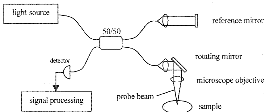
Figure 2.2 The configuration of a standard fiber-optic Michelson interferometer
