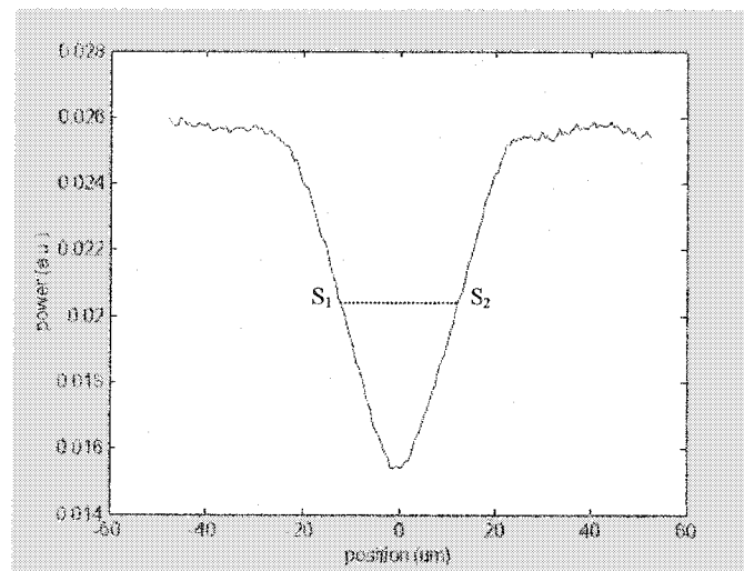
Figure 7.13 Recorded one focal spot size
