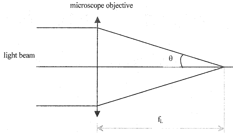
Figure 7.8 Optical path of the sample arm
