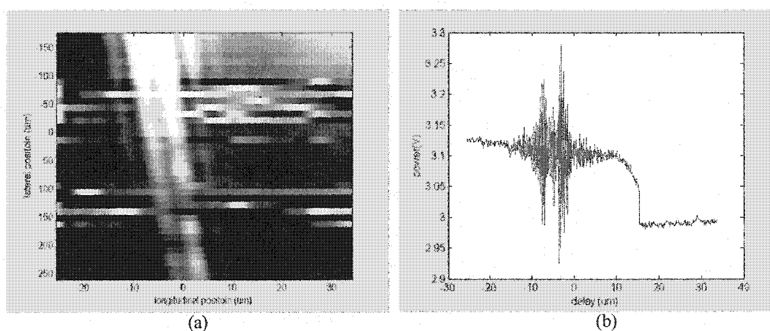
Figure 7.19 Results of the OCT scanning of the four layer sample
