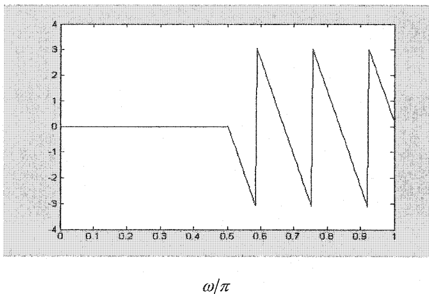
Figure 1.31: Phase of the desired filter ( Example 1.6)
