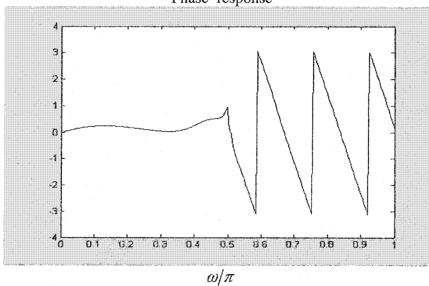
Figure 1.32: Phase of the proposed filter (max. pole radius =0.9913, Example 1.6)
