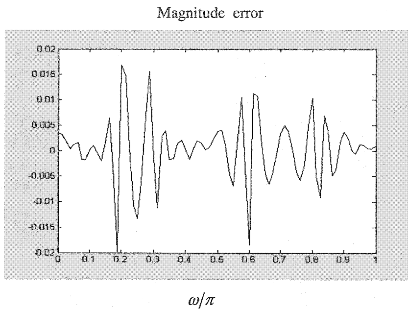
Figure 1.12: Magnitude error of the IIR filter (Gauss-Newton method)
