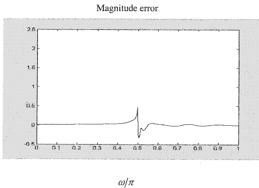
Figure 1.35: Magnitude error of the IIR filter (Proposed algorithm 2, table 1.4)
