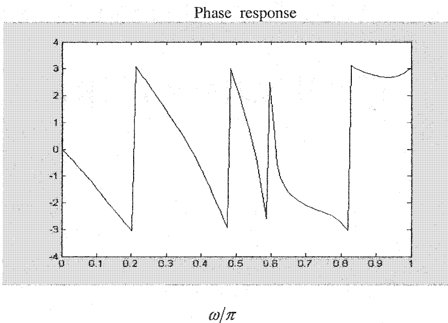
Figure 1.66: Phase of the proposed filter (max. pole radius=0.9800, Example 1.11)
