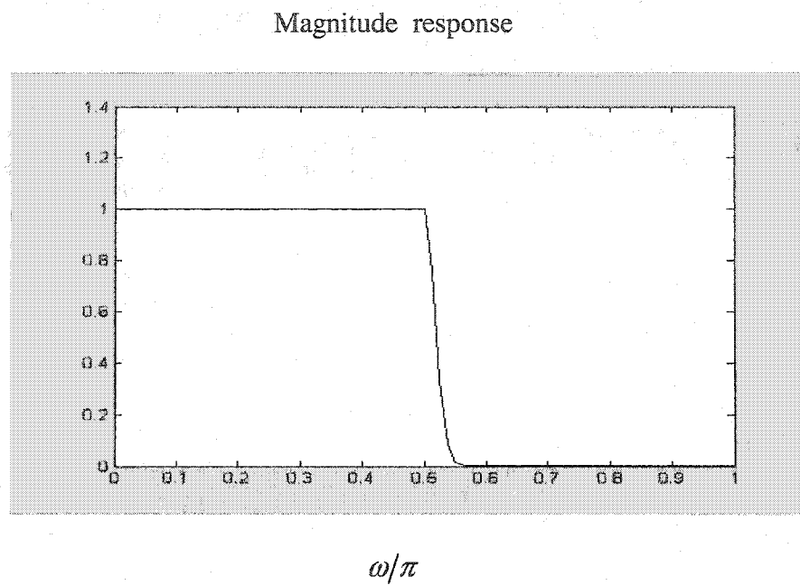
Figure 1.4: Magnitude of the proposed filter (Example 1.2)
