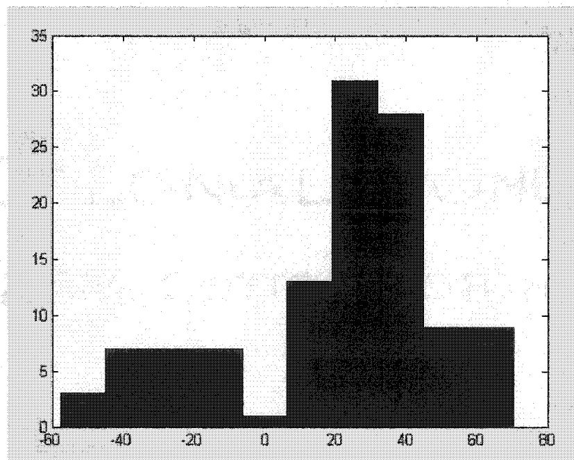
Figure 2.6: Histogram of mmtlcobb1
