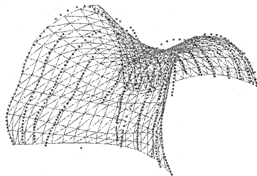
Figure 3.3: Surface approximation to figure 3.2 with a 10x4 control points set
