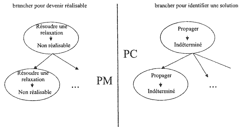
Figure 2.1: Branch and bound programmation mathématique (PM) vs programmation par contraintes (PC)
